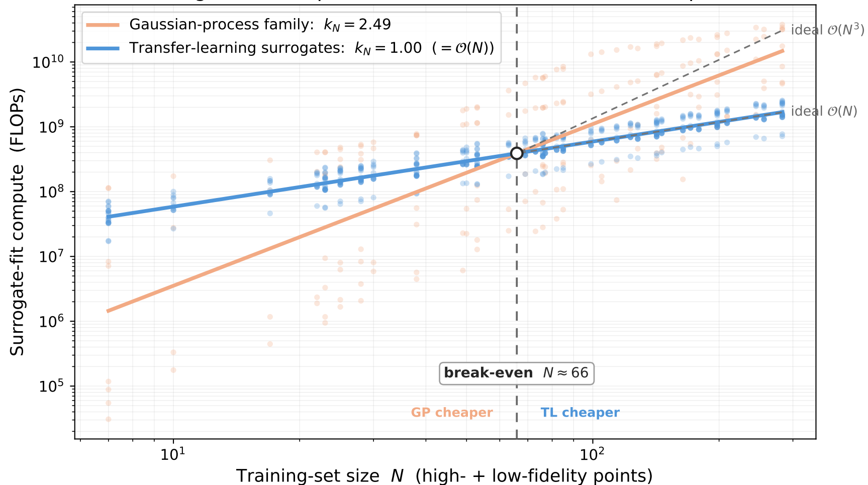
Surrogate-fit compute scales with the number of data points
