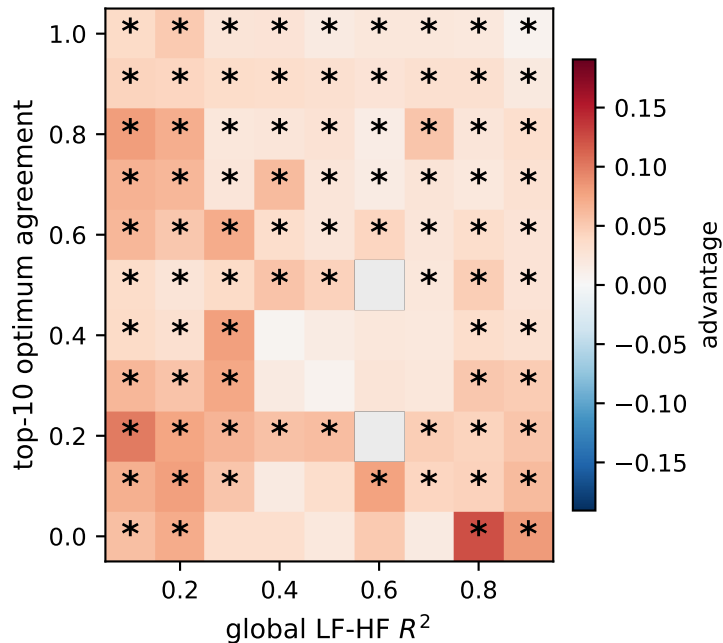
TL vs MFGP variants (red: TL better, blue: MFGP variants better)
