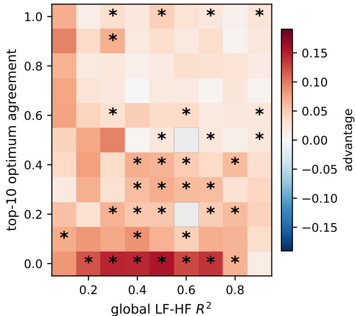
MFGP variants vs MFGP baseline (red: MFGP variants better, blue: MFGP baseline better)
