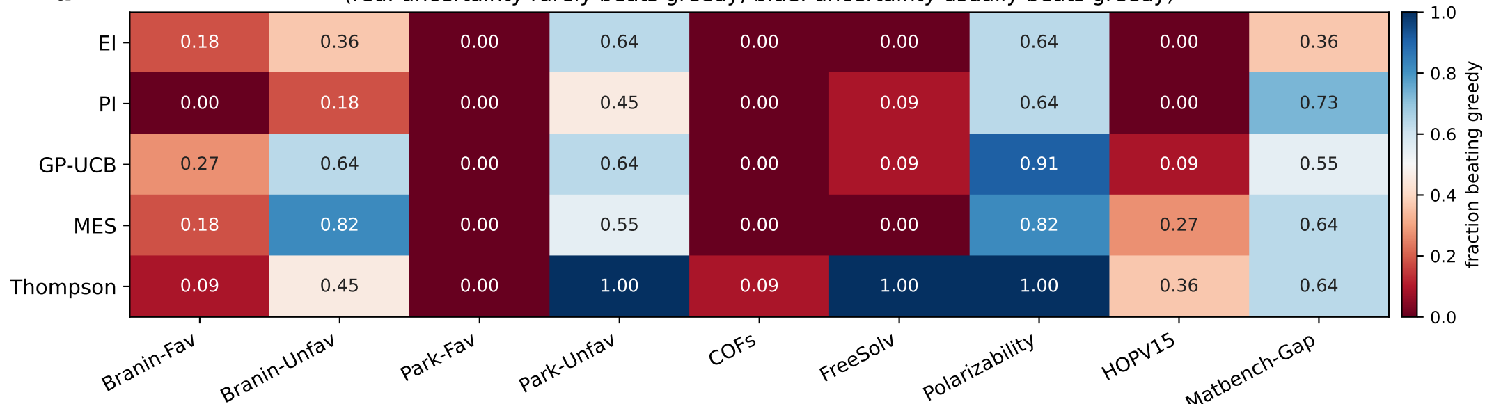
Fraction of 11 transfer-learning surrogates on which each uncertainty acquisition beats greedy (red: uncertainty rarely beats greedy; blue: uncertainty usually beats greedy)
