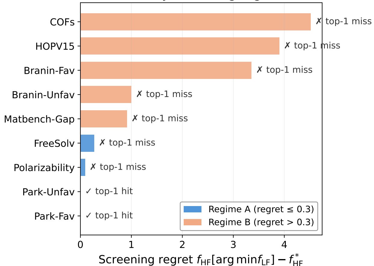
b LF-only screening regret
