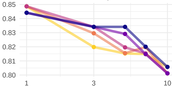
accuracy
