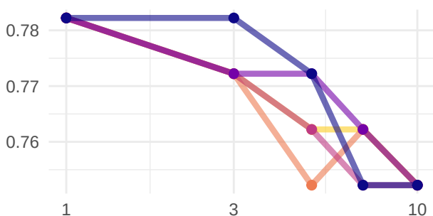
recall
