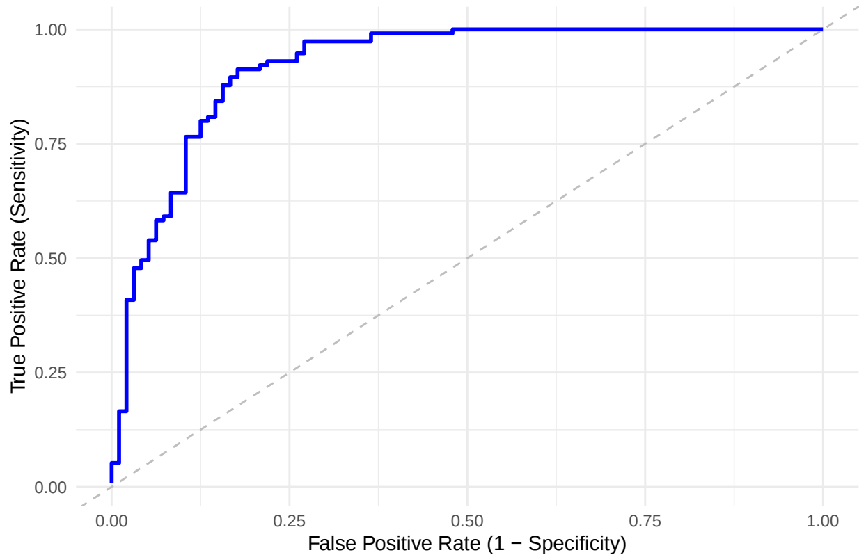
ROC Curve – SuperLearner
