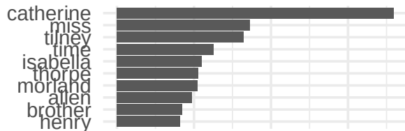
Northanger Abbey
