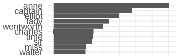
Persuasion
