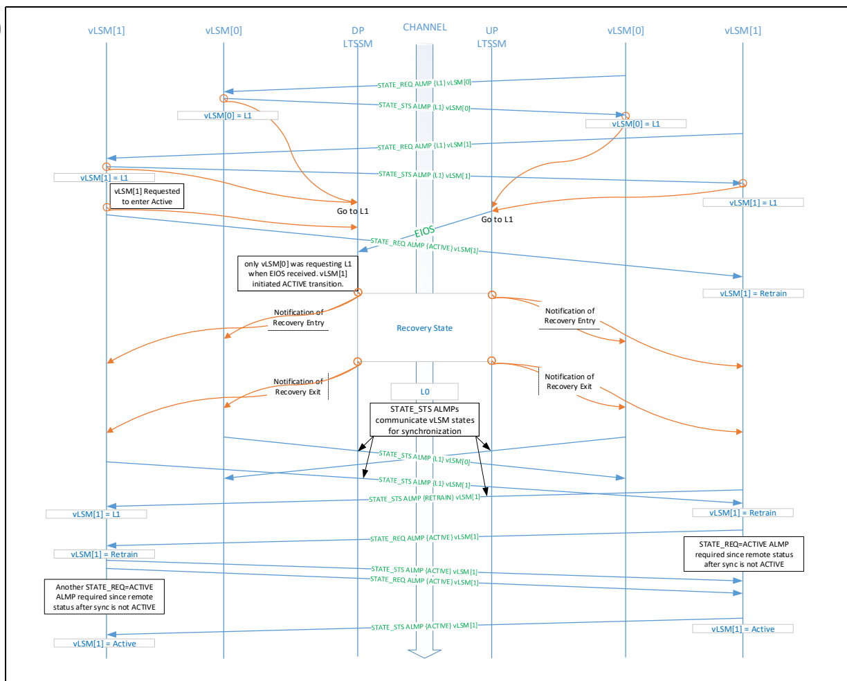
Figure 5-17. L1 Abort Example
