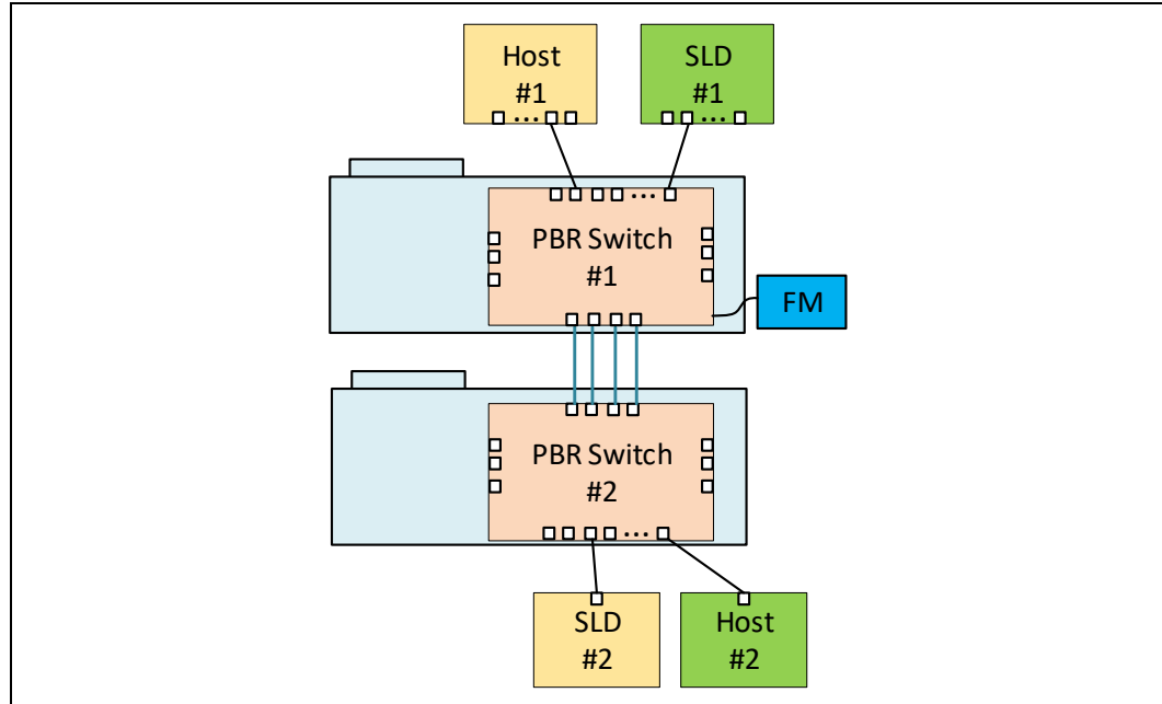
Figure 14-7. Example Topology for Two PBR Switches
