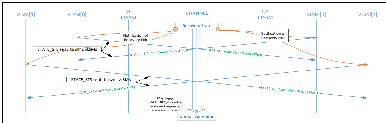
Figure 5-10. CXL Recovery Exit Example Flow
