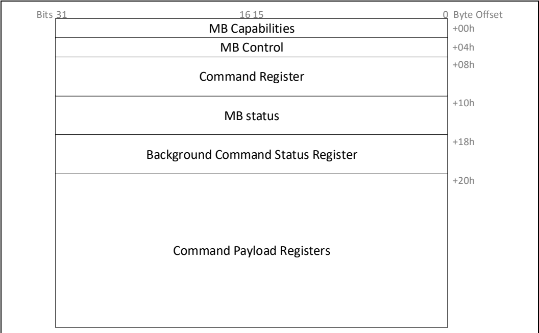
Figure 8-14. Mailbox Registers
