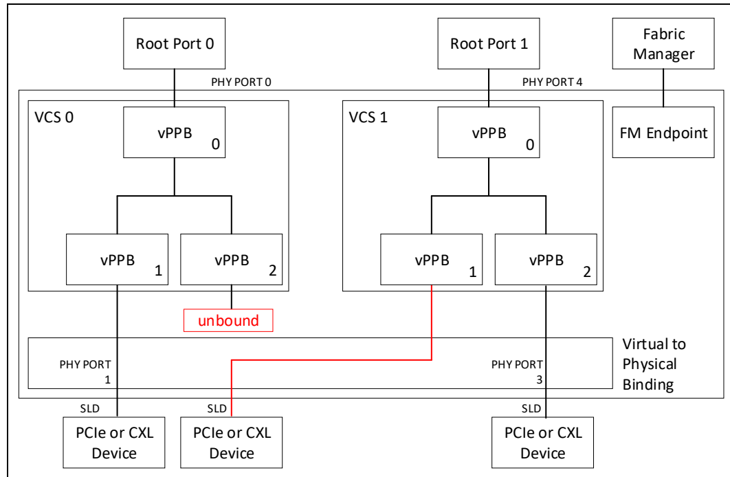
Figure 7-11. Example of CXL Switch Configuration after a Bind Command
