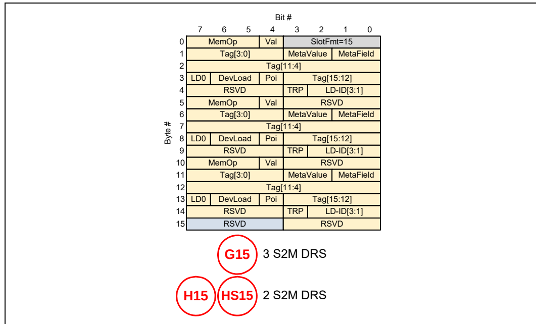
Figure 4-67. 256B Packing: G15/H15 PBR Messages
