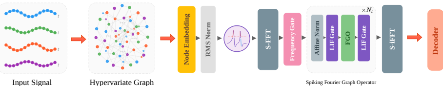
(a) The overall architecture of SpikF-GO
