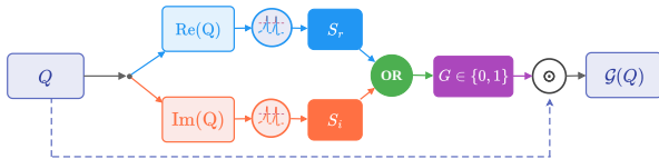
(b) Complex LIF Gate
