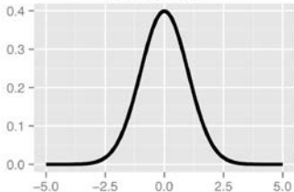
Gaussian
