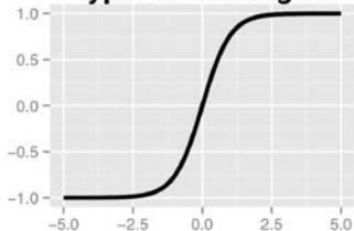
Hyperbolic Tangent
