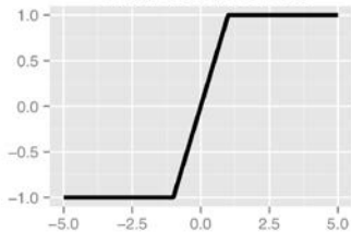
Saturated Linear
