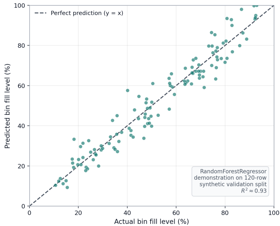
Figure 6.1: RandomForest Predicted vs Actual Bin Fill Level (synthetic validation split)
