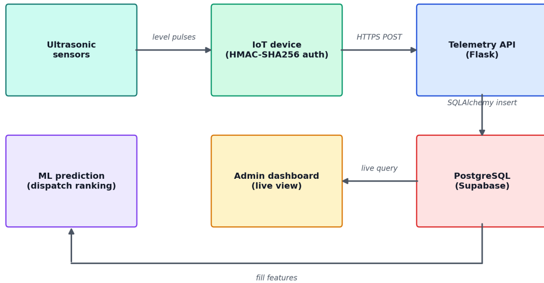
Figure 4.3: IoT Data Flow Diagram
