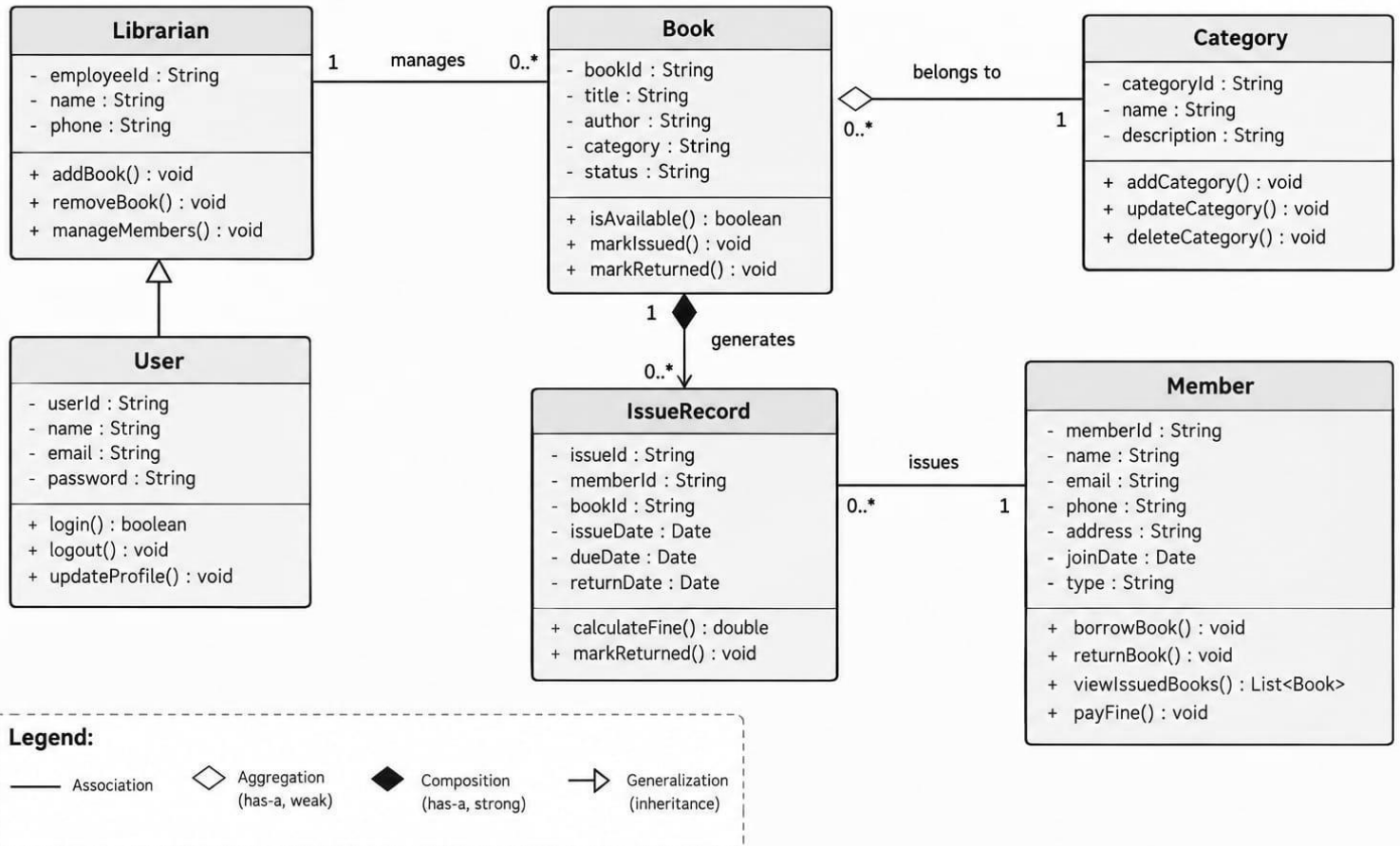
Library Management System – Class Diagram
