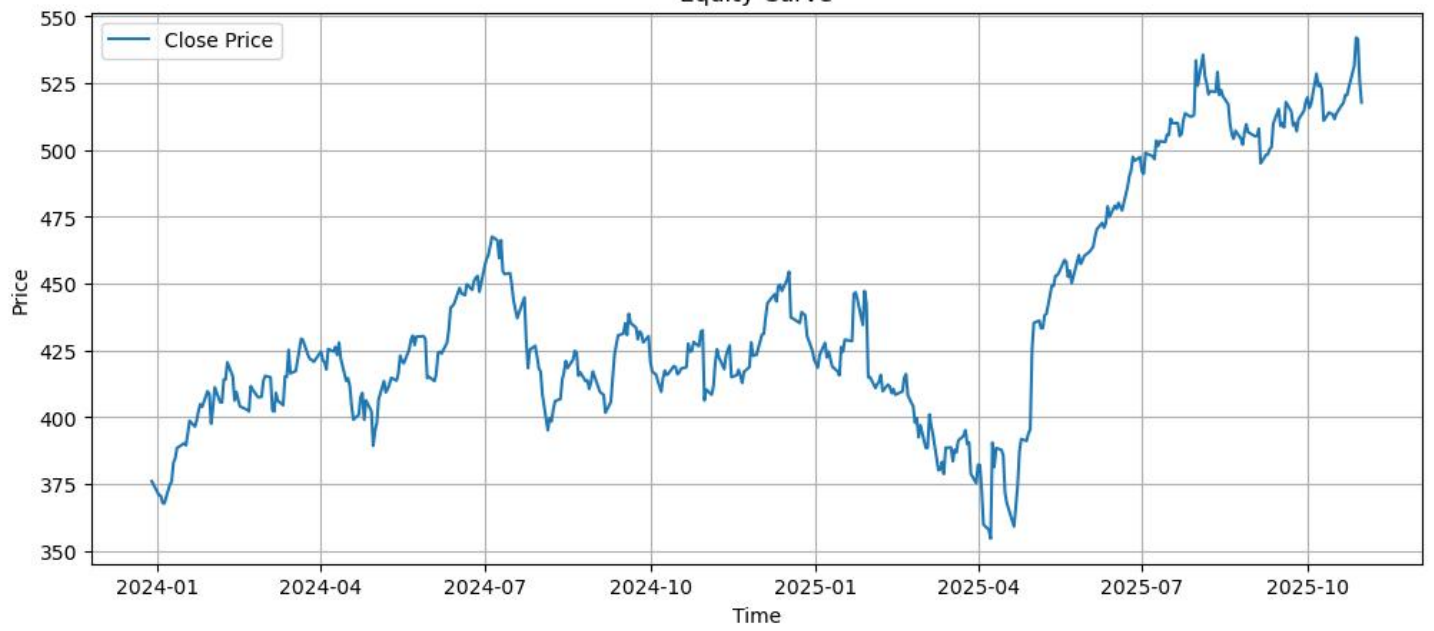
Equity Curve
