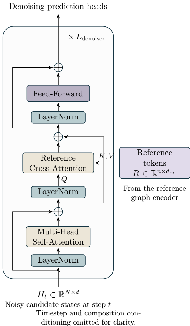
(a) Inside the denoiser
