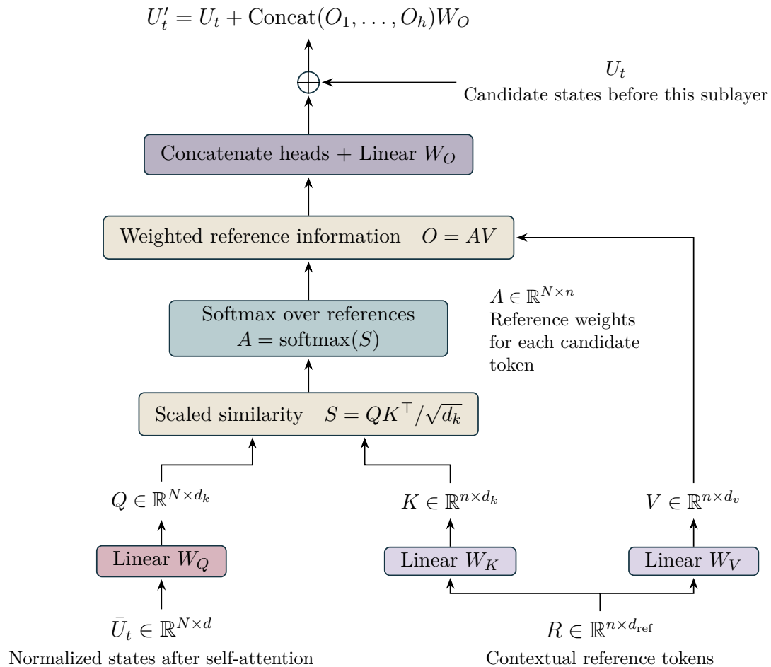
(b) Inside reference cross-attention
