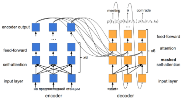
Fig. 12. Unfolded network architecture of the transformer [13]
