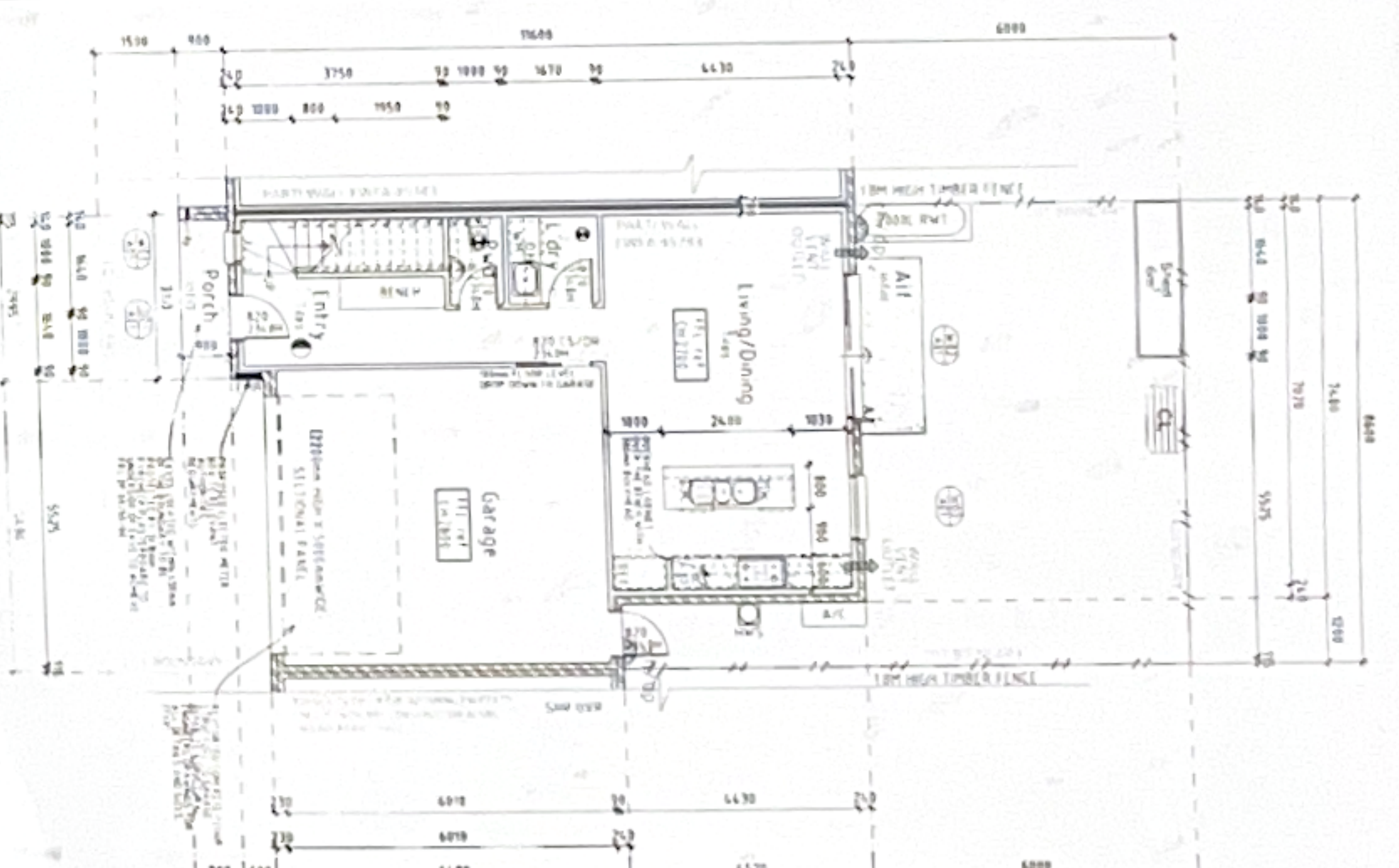
UNIT 3-11 (TYPE B) FLOOR PLAN Scale: 1:100
