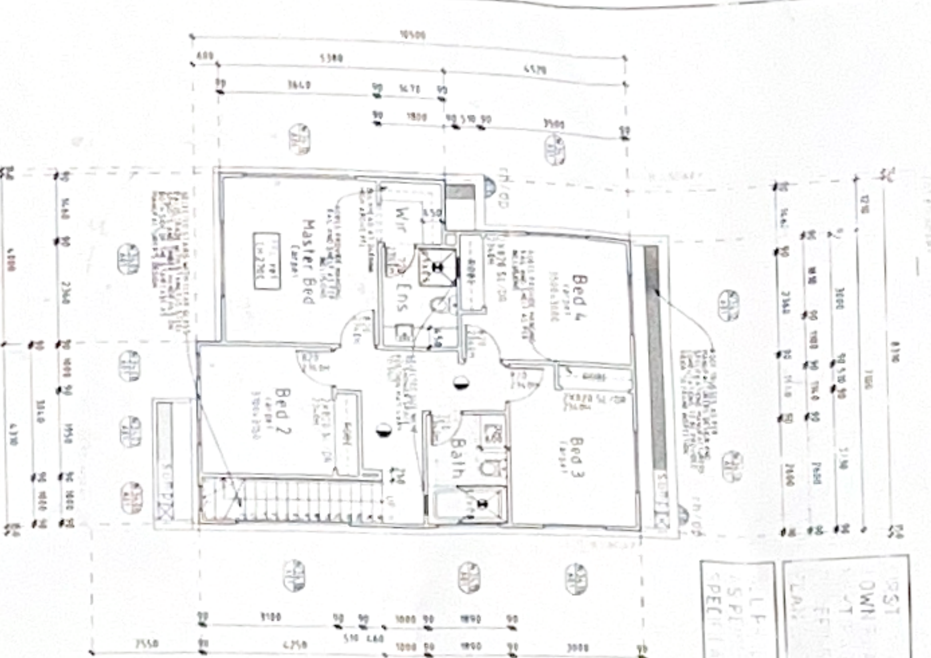
UNIT 34 (TYPE B.1) FLOOR PLAN Scale: 1:100
