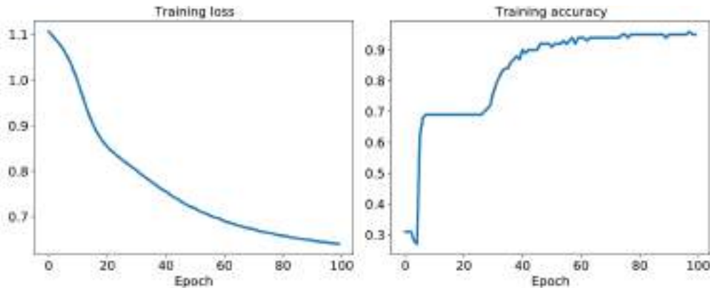
Figure 12.9: Training loss and accuracy curves
