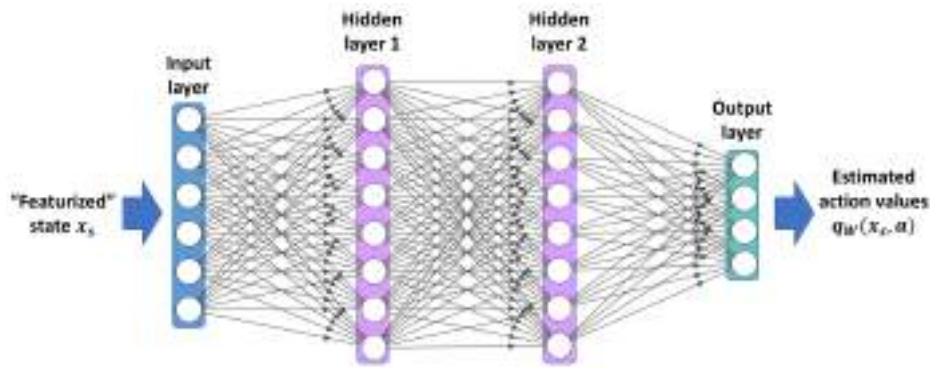
Figure 19.10: An example of a DQN
