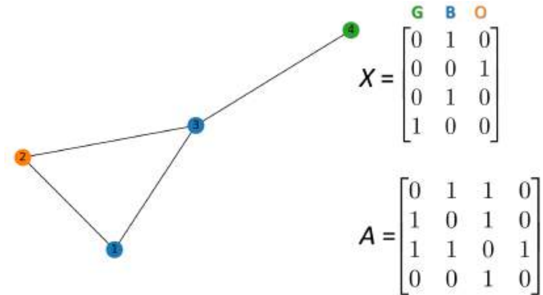
Figure 18.6: A representation of a graph
