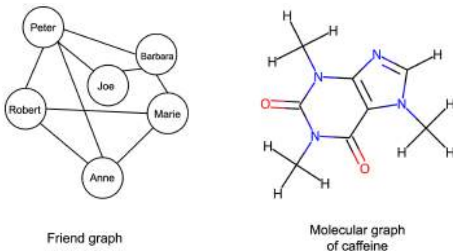
Figure 18.2: Two examples of undirected graphs
