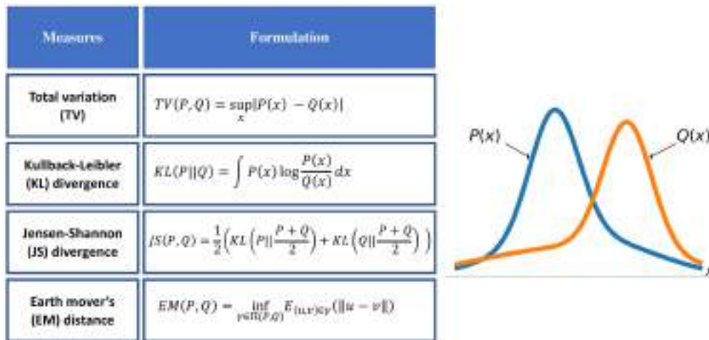
Figure 17.18: Methods to measure the dissimilarity between distributions P and Q
