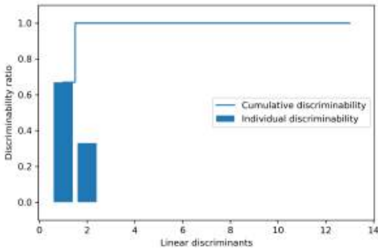
Figure 5.9: The top two discriminants capture 100 percent of the useful information
