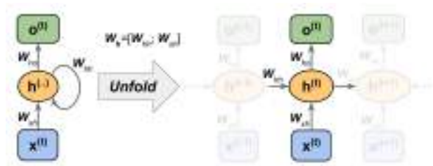
Figure 15.5: Applying weights to a single-layer RNN
