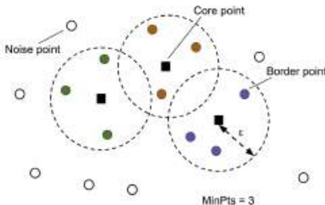
Figure 10.13: Core, noise, and border points for DBSCAN
