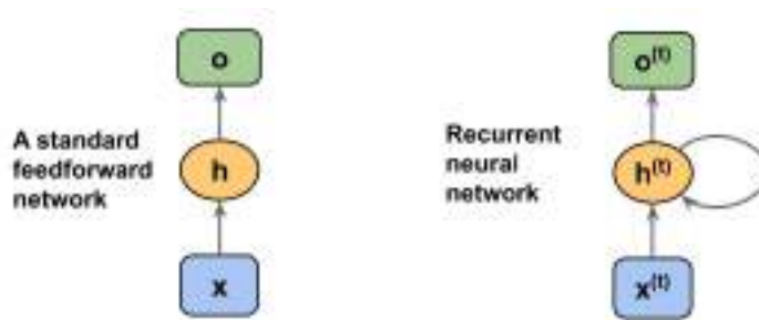
Figure 15.3: The dataflow of a standard feedforward NN and an RNN
