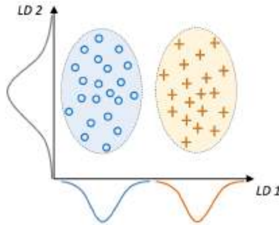
Figure 5.8: The concept of LDA for a two-class problem
