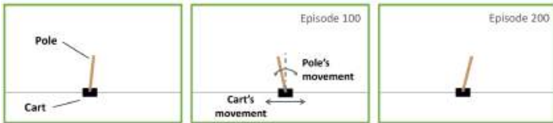
Figure 19.6: The CartPole example in Gym
