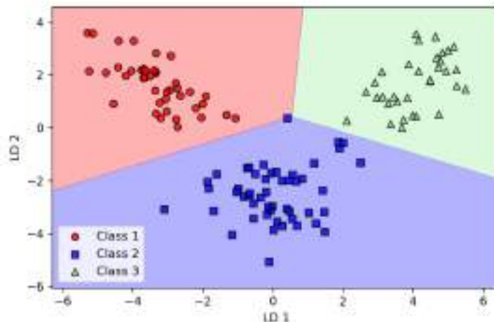
Figure 5.11: The logistic regression model misclassifies one of the classes
