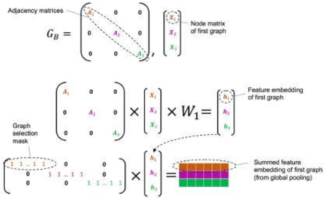
Figure 18.10: How to deal with varying graph sizes
