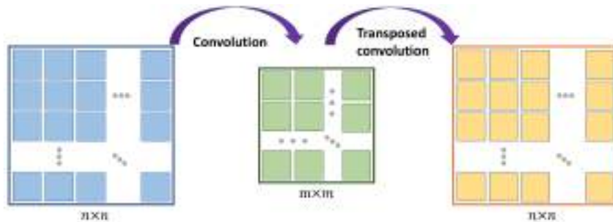
Figure 17.12: Transposed convolution
