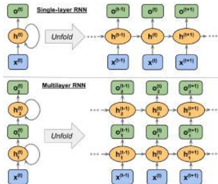
Figure 15.4: Examples of an RNN with one and two hidden layers
