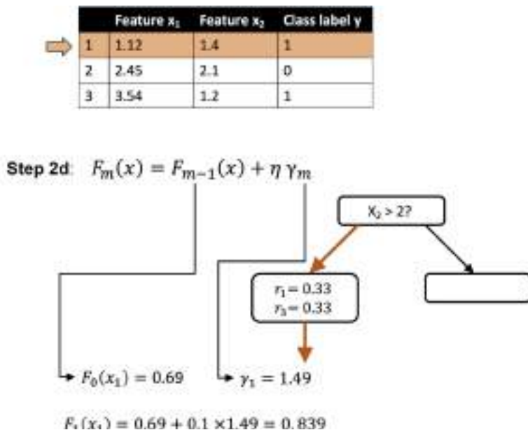
Figure 7.15: The update of the previous model shown in the context of the first training example
