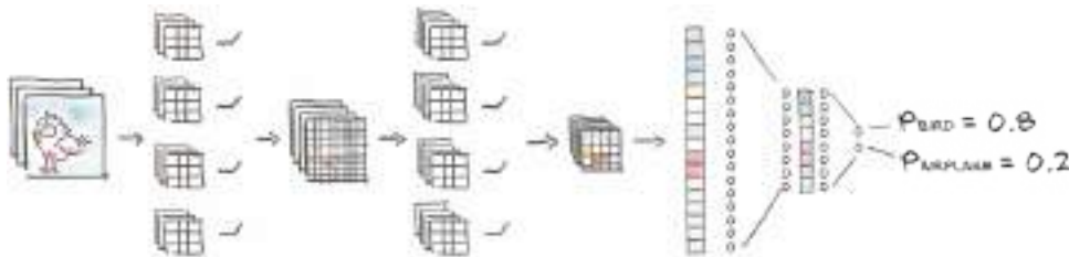
Figure 8.11 Shape of a typical convolutional network, including the one we’re building. An image is fed to a series of convolutions and max pooling modules and then straightened into a 1D vector and fed into fully connected modules.
