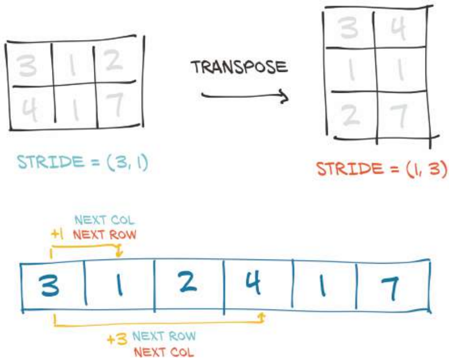
Figure 3.6 Transpose operation applied to a tensor.
