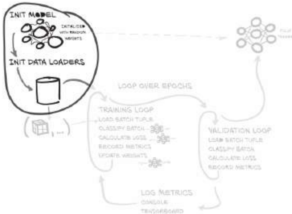
Figure 13.3 The training and validation script we will implement in this chapter, with a focus on the preloop variable initialization.
