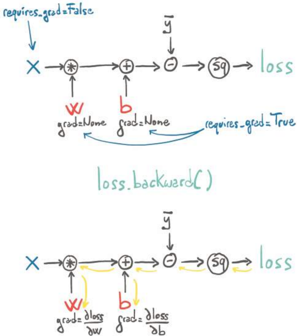
Figure 5.11 The forward graph and backward graph of the model as computed with autograd.
