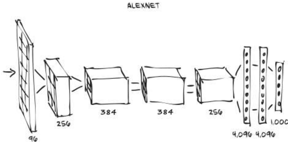
Figure 2.3 The AlexNet architecture (numbers denote outputs at each layer).
