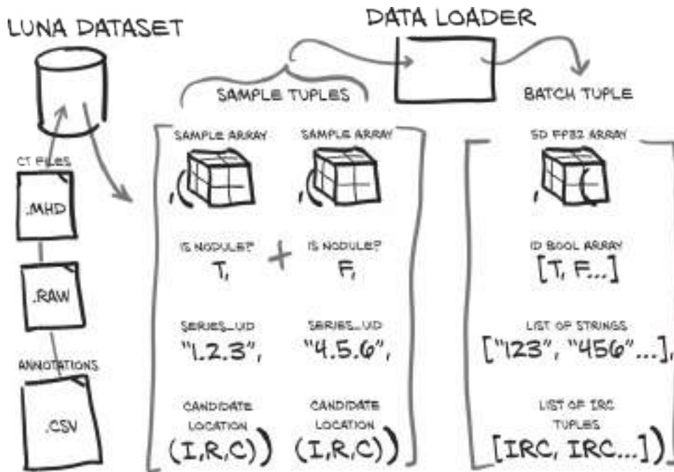
Figure 13.4 Sample tuples being collated into a single batch tuple inside a data loader.
