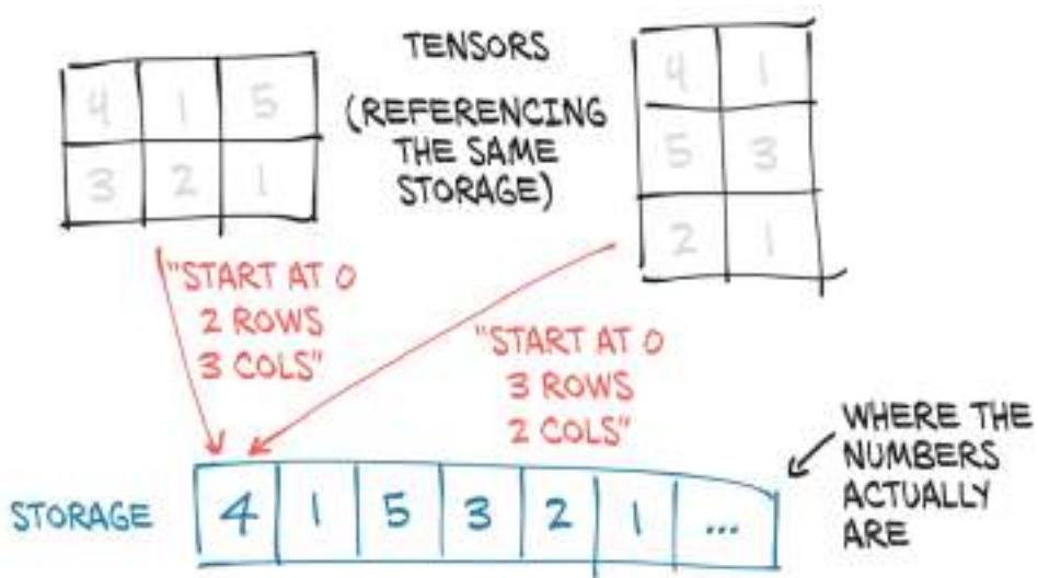
Figure 3.4 Tensors are views of a Storage instance.
