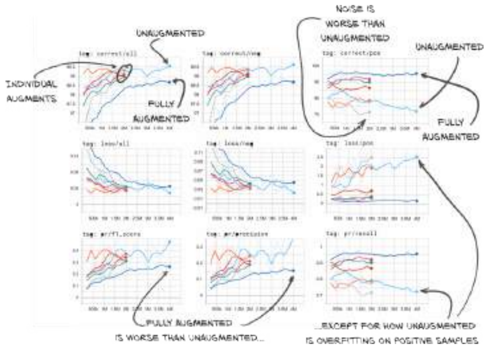
Figure 14.22 Percent correctly classified, loss, F1 score, precision, and recall for the validation set from networks trained with a variety of augmentation schemes.
