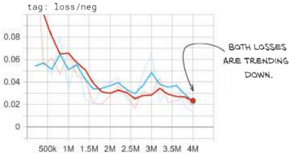
Figure 14.19 Our negative loss showing no signs of overfitting.
