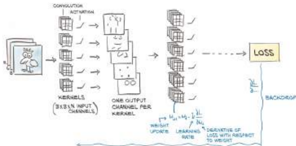
Figure 8.8 The process of learning with convolutions by estimating the gradient at the kernel weights and updating them individually in order to optimize for the loss.
