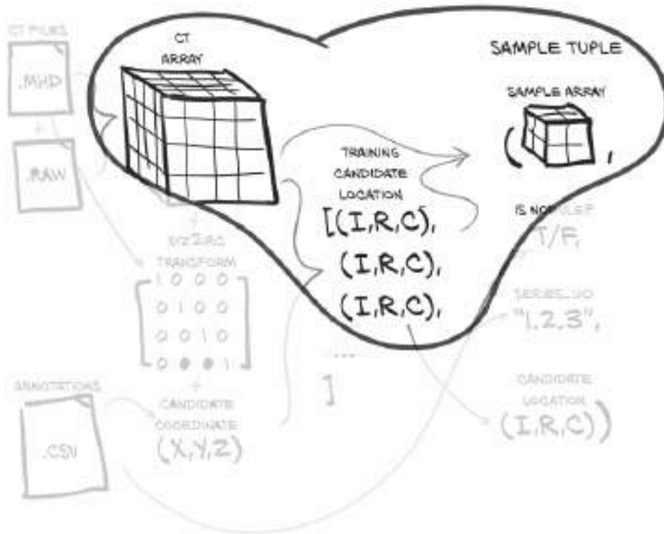
Figure 12.9 Cropping a candidate sample out of the larger CT voxel array using the candidate center's array coordinate information (Index,Row,Column)
