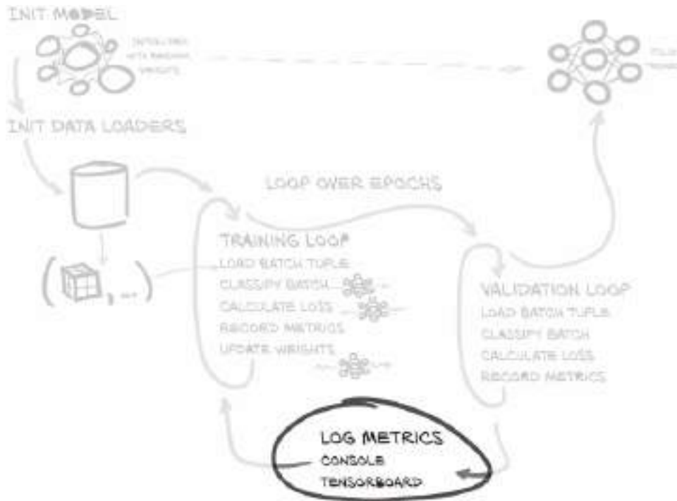
Figure 13.9 The training and validation script we will implement in this chapter, with a focus on the metrics logging at the end of each epoch.
