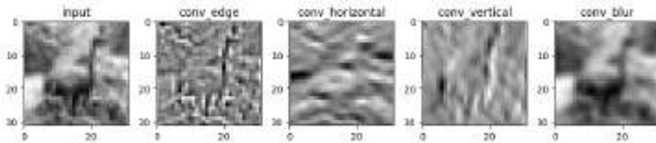
Figure 8.7 Different kernel examples for detecting different features. We have hardcoded these examples for illustration purposes but in reality, the model will learn the appropriate kernels for the task at hand.
