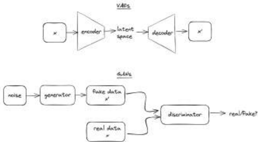
Figure 10.1 Architectural comparison of variational autoencoders (VAE) and generative adversarial networks (GAN). VAEs utilize latent space to generate new samples, while GANs use a generator/discriminator pair to create new data.
