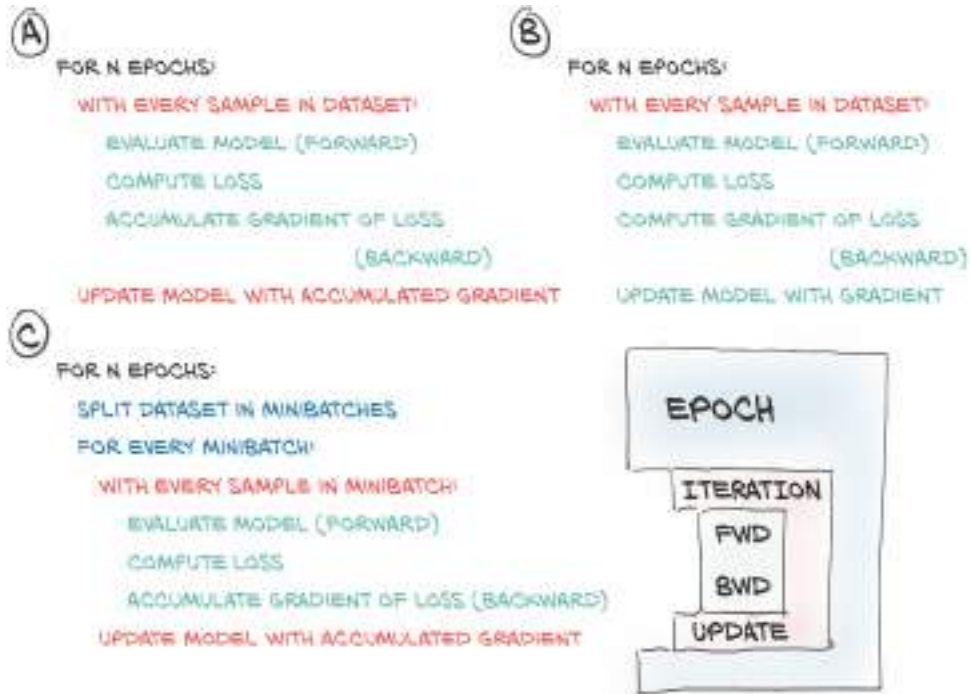
Figure 7.12 Training loops: (A) averaging updates over the whole dataset; (B) updating the model at each sample; (C) averaging updates over minibatches.
