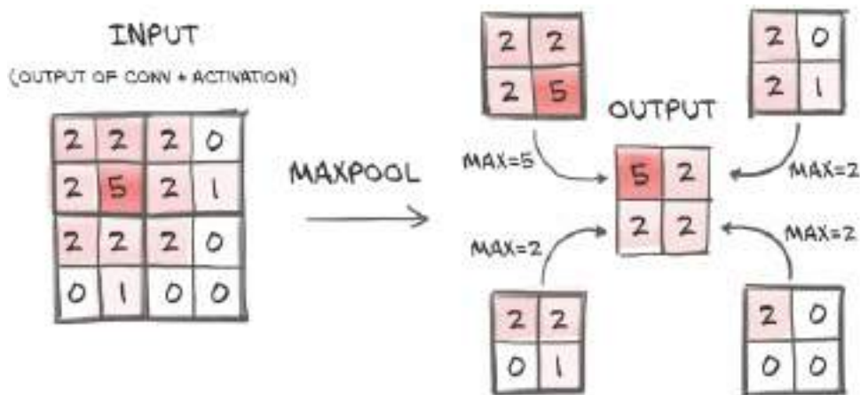
Figure 8.9 Max pooling in detail.
