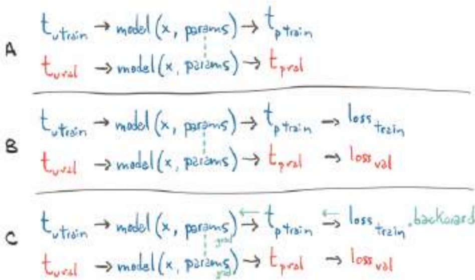
Figure 5.16 Diagram showing how gradients propagate through a graph with two losses when .backward is called on one of them.
