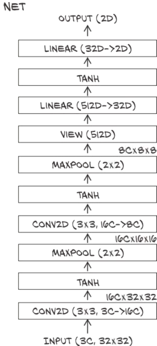
Figure 8.12 Our baseline convolutional network architecture.
