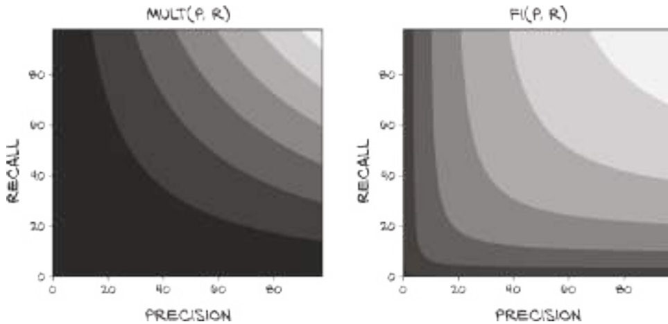
Figure 14.13 Computing the final score with mult(p, r) .
