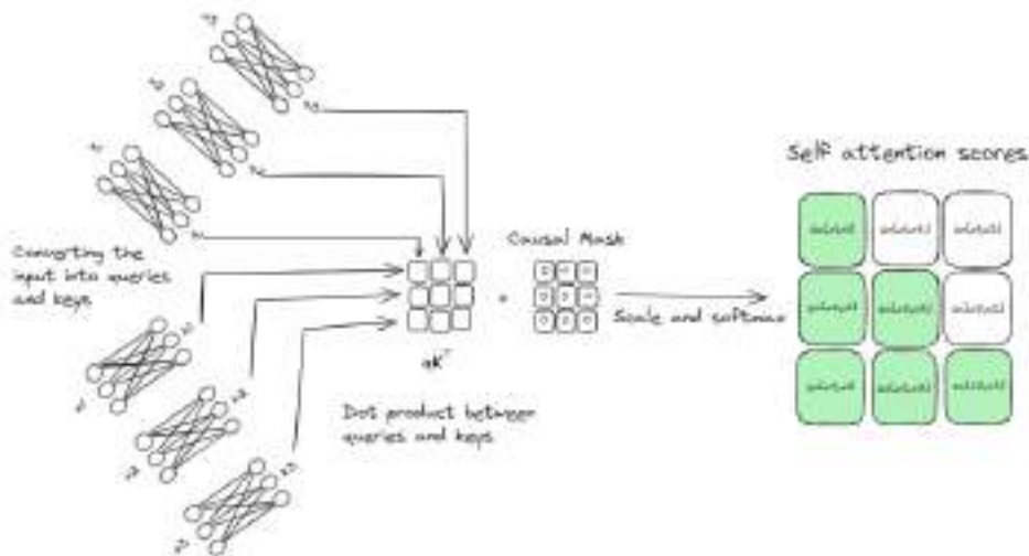
Figure 9.8 Full causal self-attention mechanism
