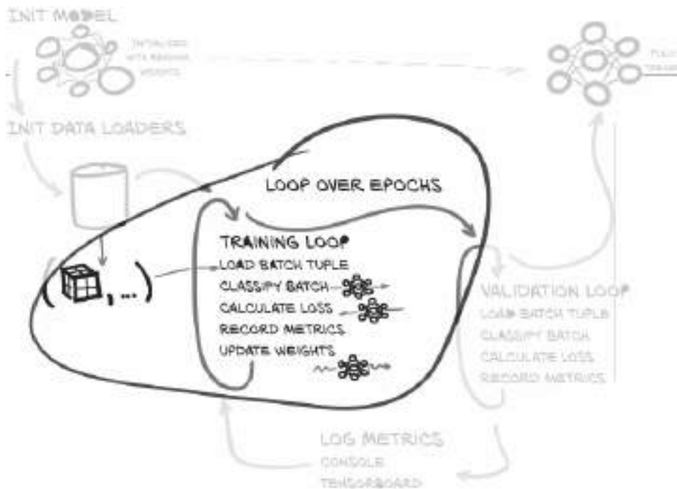
Figure 13.7 The training and validation script we will implement in this chapter, with a focus on the nested loops over each epoch and batches in the epoch.
