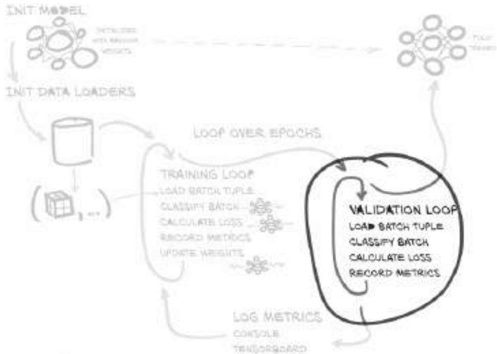
Figure 13.8 The training and validation script we will implement in this chapter, with a focus on the per-epoch validation loop.
