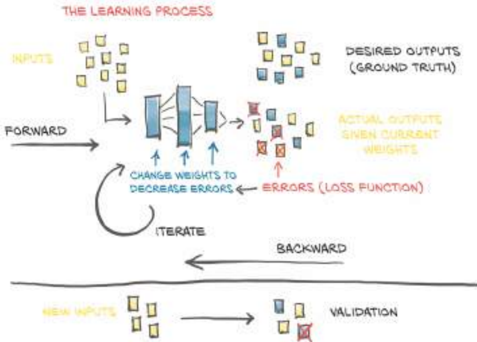
Figure 5.2 Our mental model of the learning process.
