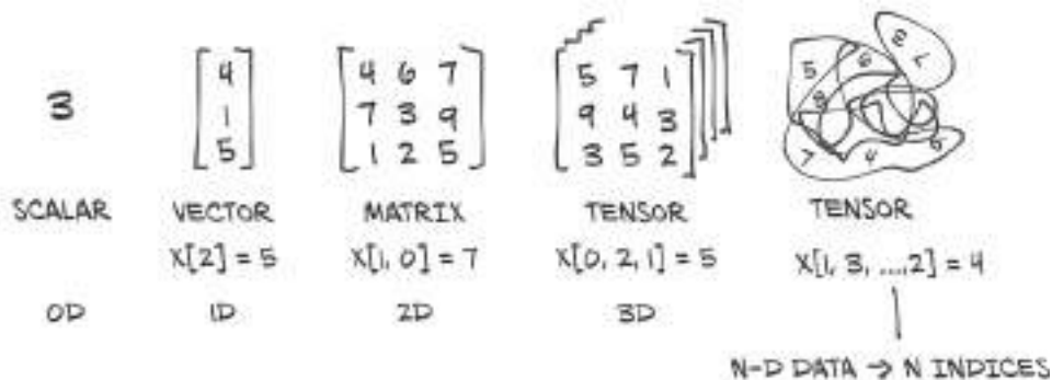
Figure 3.2 Tensors are the building blocks for representing data in PyTorch. Scalars, vectors, and matrices can also all be considered tensors.
