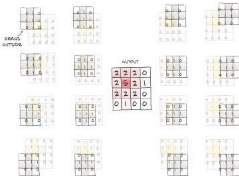
Figure 8.4 Padding=1 wraps 0s around all sides of the input to preserve the image size in the output.
