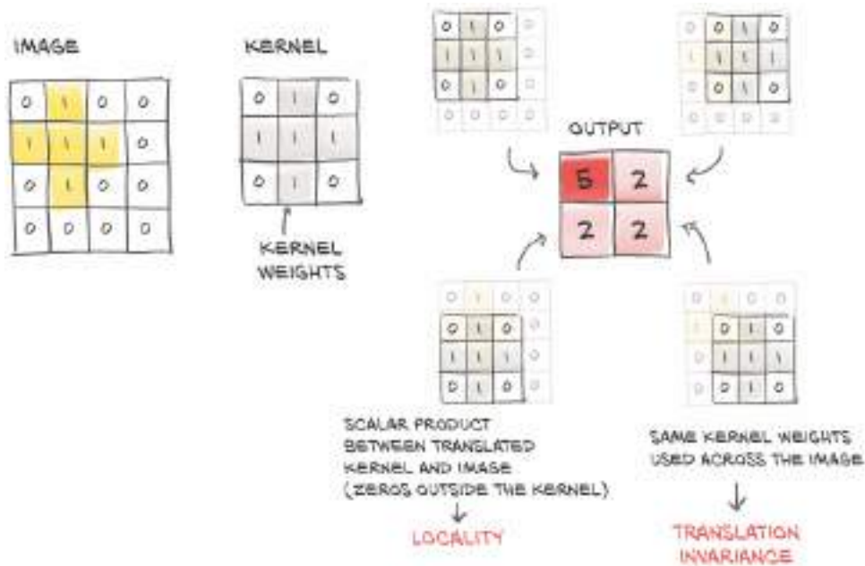
Figure 8.1 Convolution: locality and translation invariance.
