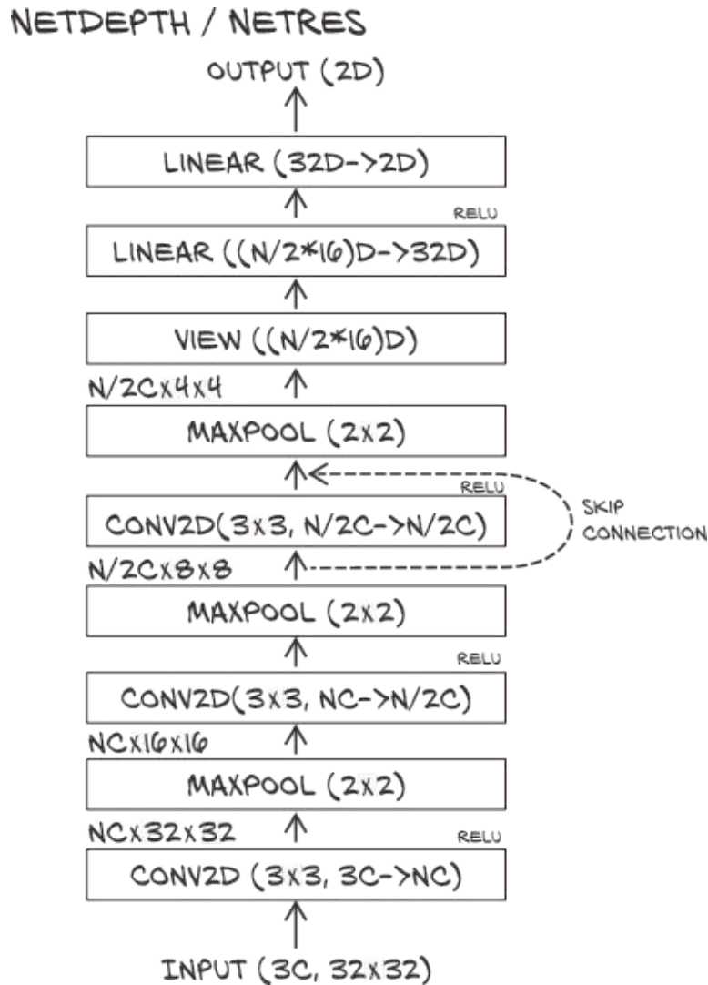
Figure 8.14 The architecture of our network with three convolutional layers. The skip connection is what differentiates NetRes from NetDepth.
