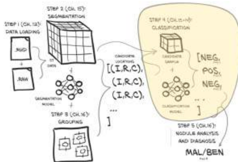
Figure 13.1 Our end-to-end project to detect lung cancer, with a focus on this chapter's topic: step 4, classification.
