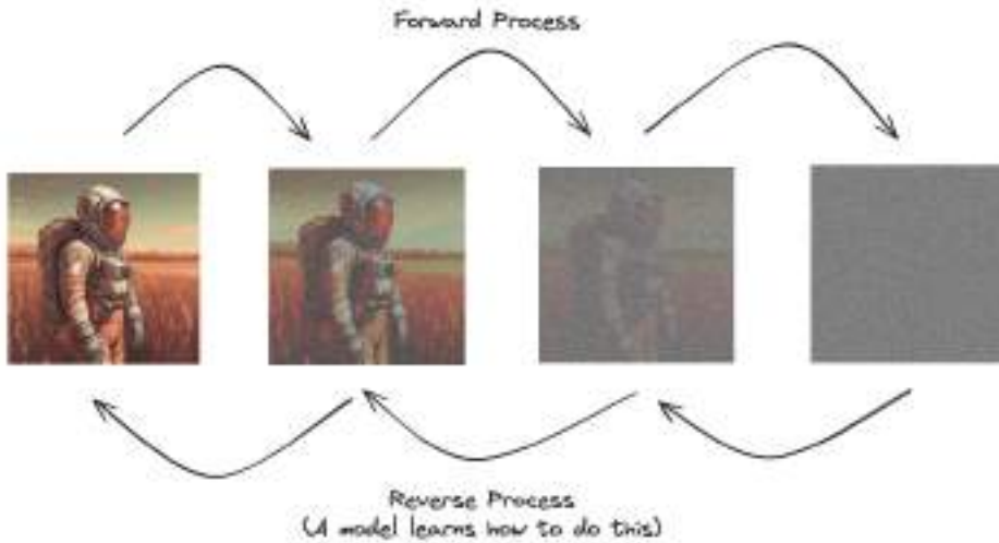
Figure 10.3 Forward and reverse process of diffusion models on an image
