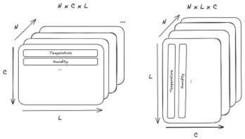
Figure 4.6 The dimensions N \times C \times L (left) vs. N \times L \times C (right) visualized.
