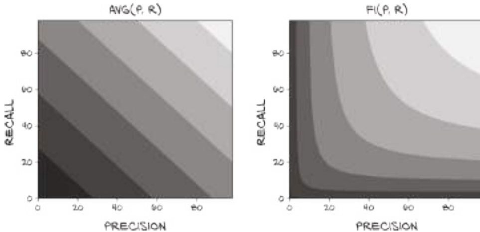
Figure 14.11 Computing the final score with \text{avg}(p, r) . Lighter values are closer to 1.0 and darker values are closer to 0.0.
