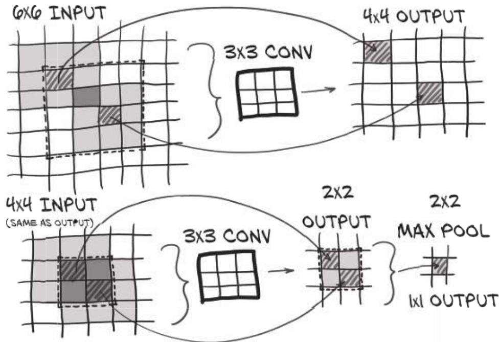
Figure 13.6 The convolutional architecture of a LunaModel block consisting of two 3 \times 3 convolutions followed by a max pool. The final pixel has a receptive field of 6 \times 6 .
