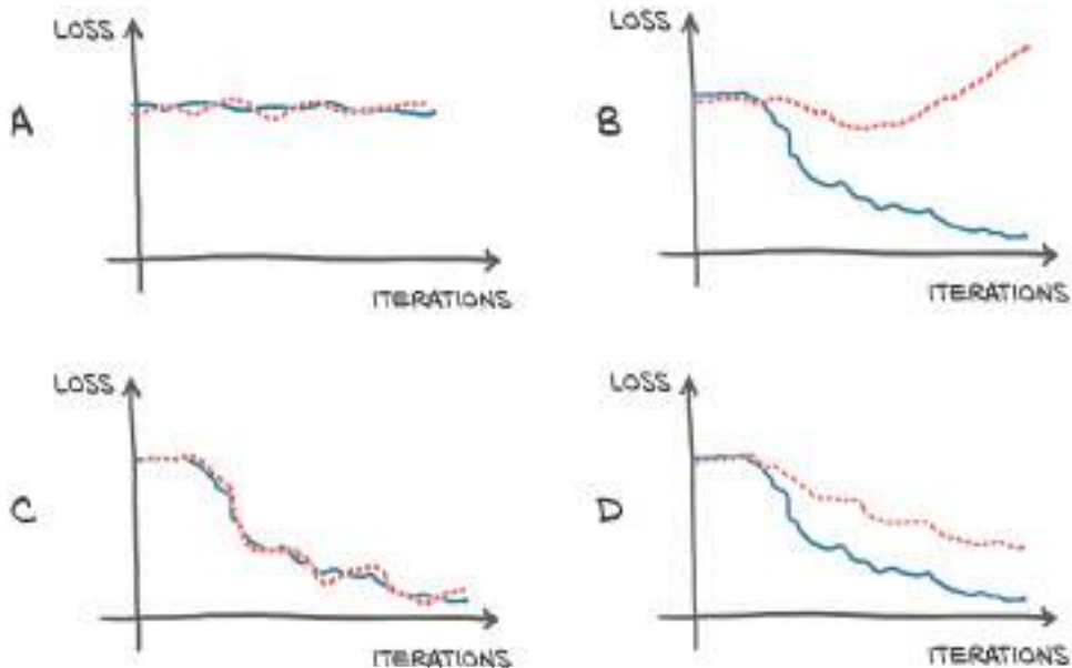
Figure 5.15 Overfitting scenarios when looking at the training (solid line) and validation (dotted line) losses. (A) Training and validation losses do not decrease; the model is not learning due to no information in the data or insufficient capacity of the model. (B) Training loss decreases while validation loss increases: overfitting. (C) Training and validation losses decrease exactly in tandem. Performance may be improved further as the model is not at the limit of overfitting. (D) Training and validation losses have different absolute values but similar trends: overfitting is under control.
