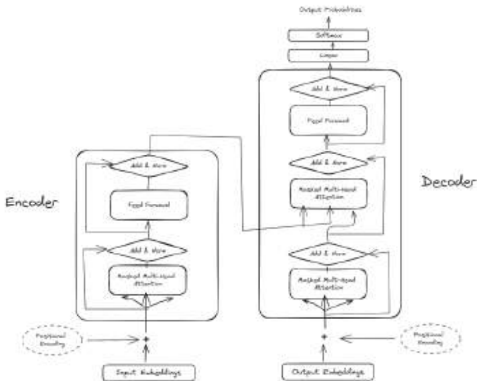
Figure 9.13 Diagram of the transformer architecture from the original paper "Attention is All You Need". The encoder is on the left and the decoder is on the right. The encoder output is fed into the decoder as the key and value for the multi-head attention mechanism.
