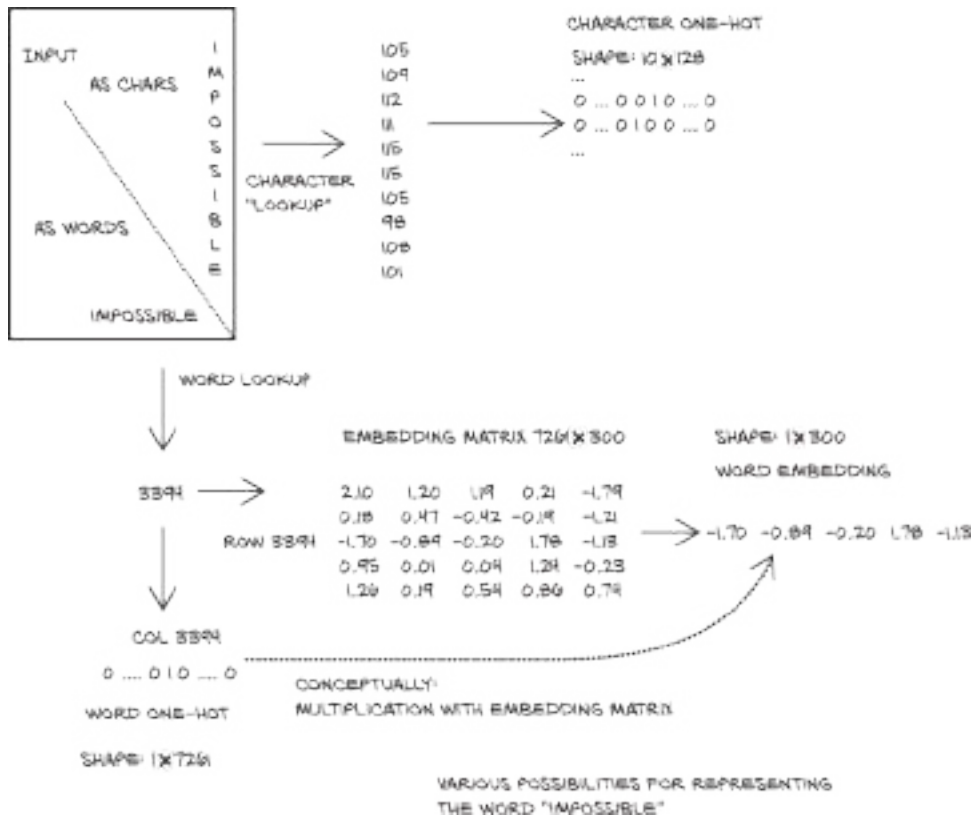
Figure 4.7 Three ways to encode a word.
