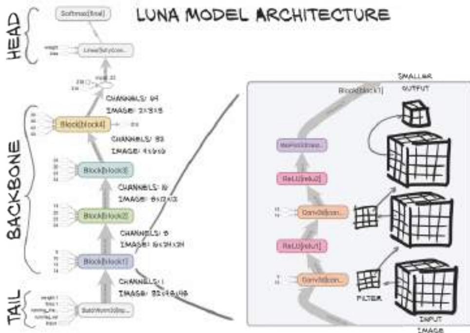
Figure 13.5 The architecture of the LunaModel class consisting of a batch-normalization tail, a four-block backbone, and a head comprised of a linear layer followed by softmax.
