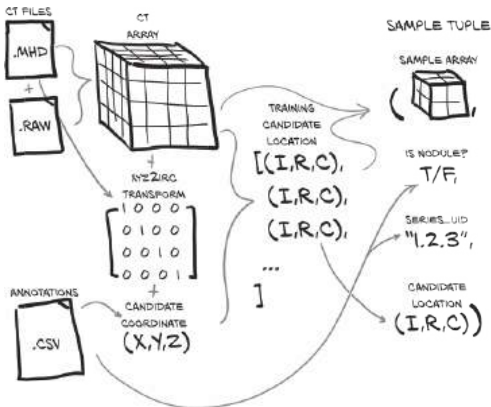
Figure 12.2 The data transforms required to make a sample tuple. These sample tuples will be used as input to our model training routine.
