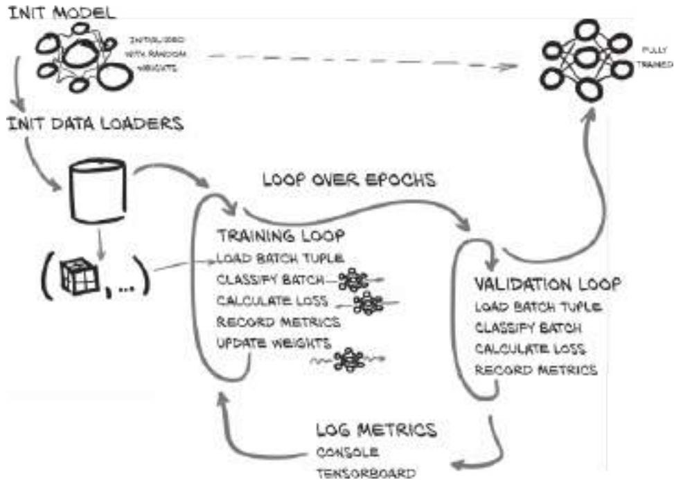
Figure 13.2 The training and validation script we will implement in this chapter.
