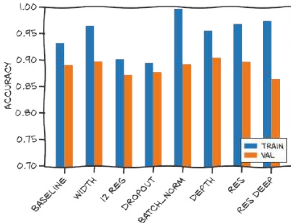
Figure 8.16 The modified networks all perform similarly.
