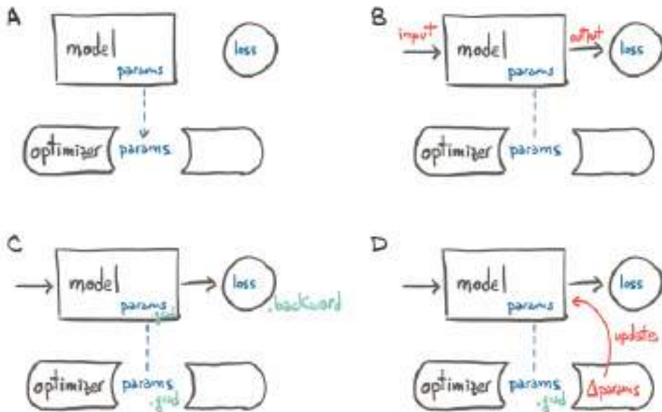
Figure 5.12 (A) Conceptual representation of how an optimizer holds a reference to parameters. (B) After a loss is computed from inputs, (C) a call to .backward leads to .grad being populated on parameters. (D) At that point, the optimizer can access .grad and compute the parameter updates.
