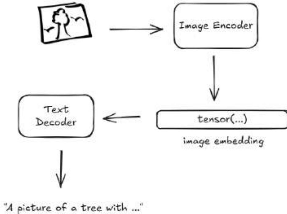
Figure 2.9 Conceptual diagram of BLIP caption generation.
