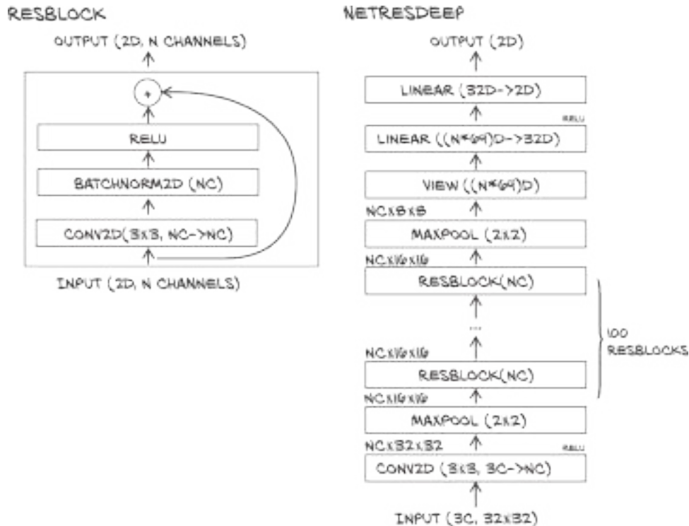
Figure 8.15 Our deep architecture with residual connections. On the left, we define a simplistic residual block. We use it as a building block in our network, as shown on the right.
