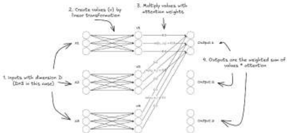
Figure 9.7 Self attention step-by-step from input to output.
