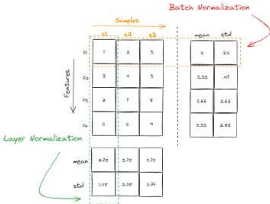
Figure 9.11 Layer normalization compared with batch normalization
