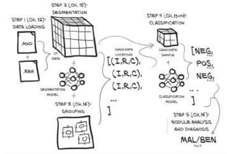
Figure 11.4 The end-to-end process of taking a full-chest CT scan and determining whether the patient has a malignant tumor.
