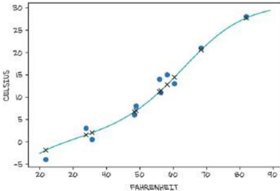
Figure 6.9 The plot of our neural network model, with input data (circles) and model output (Xs). The continuous line shows behavior captured by the neural network between samples.
