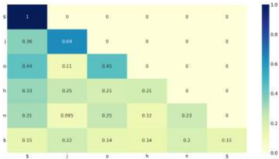
Figure 9.9 Attention weights for the name "john" visualized in a grid. Each row of values sum to 1. The darker the color, the higher the attention weight.
