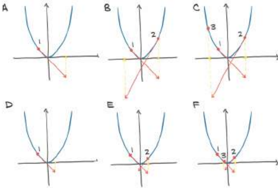
Figure 5.9 Top: Diverging optimization on a convex function (parabola-like) due to large steps. Bottom: Converging optimization with small steps is the behavior we want to achieve.
