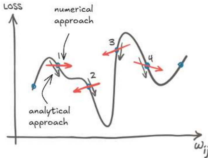
Figure 5.7 Comparing numerical vs. analytical gradient calculation: The numerical approach (arrow through points) estimates the gradient using finite differences between discrete points, while the analytical approach (arrow along the curves) calculates the exact gradient at a specific point.
