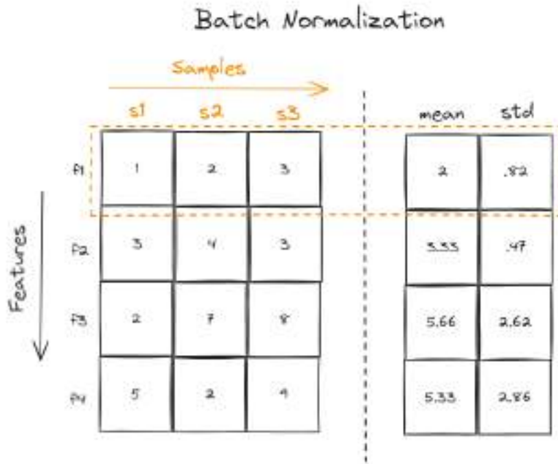
Figure 8.13 BatchNorm for 3 samples with 4 input features involves calculating the mean and standard deviation for each feature across the samples. The mean and standard deviation are then used to normalize the input features such that each feature has zero mean and unit variance.
