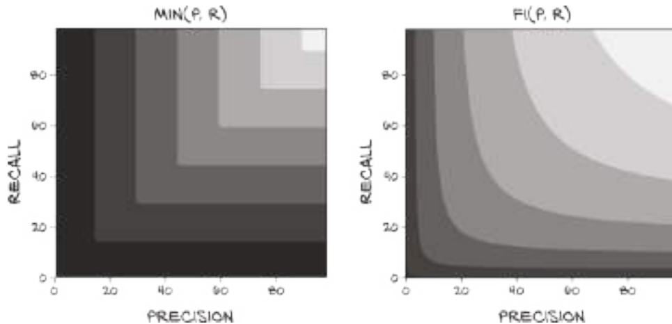
Figure 14.12 Computing the final score with \min(p, r) .
