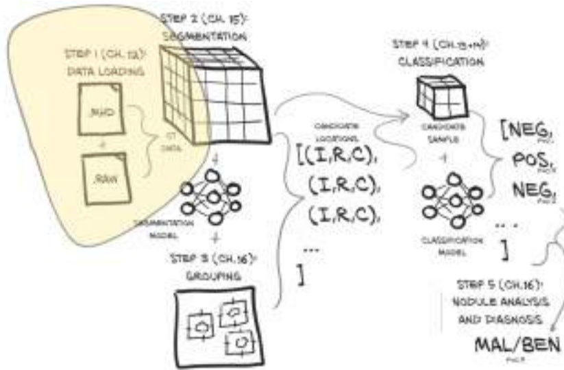
Figure 12.1 Our end-to-end lung cancer detection project, with a focus on this chapter's topic: step 1, data loading
