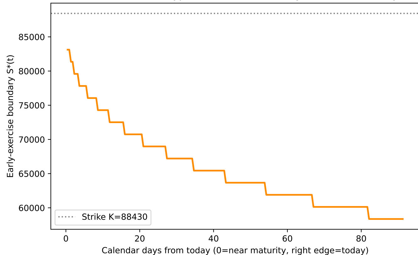
BTC-USD (volatile crypto): American Put Early-Exercise Boundary
