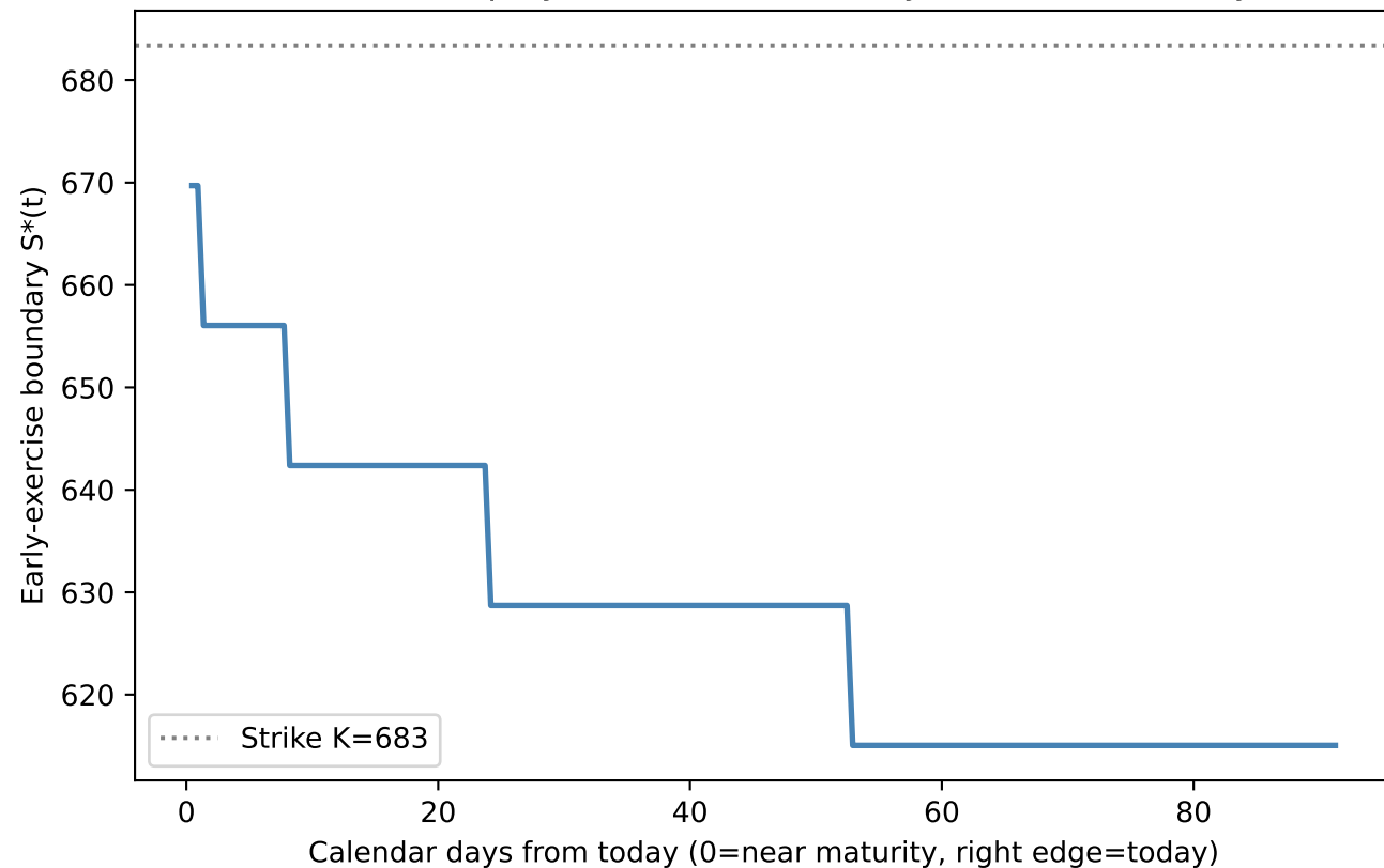
SPY (calm equity): American Put Early-Exercise Boundary
