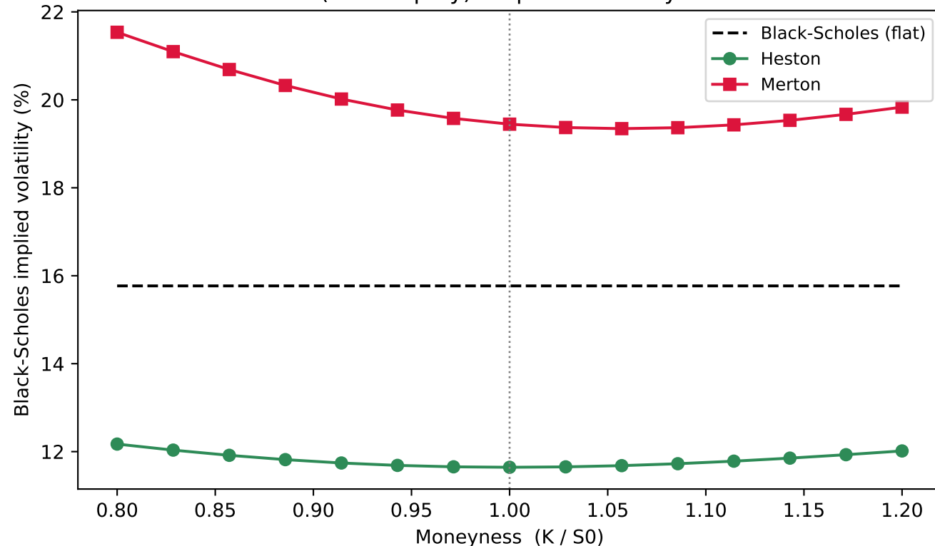
SPY (calm equity): Implied Volatility Smile
