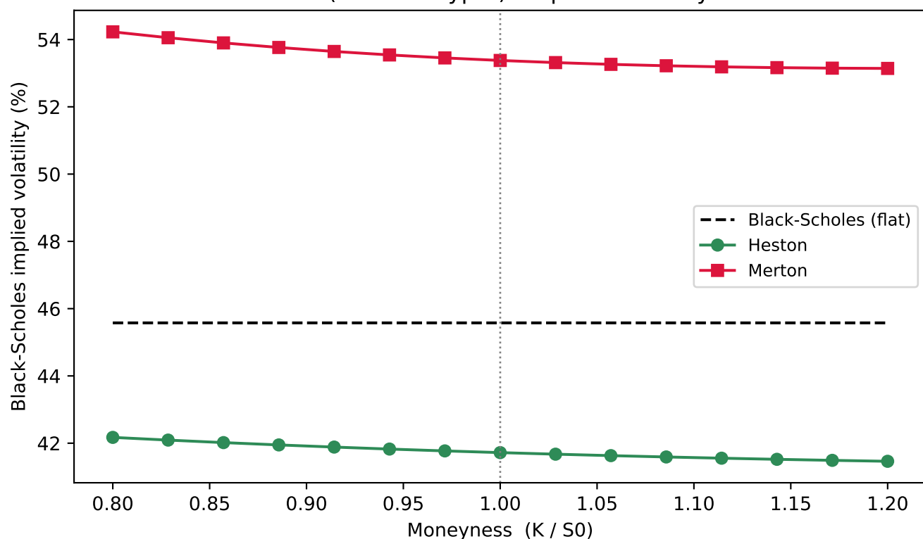
BTC-USD (volatile crypto): Implied Volatility Smile
