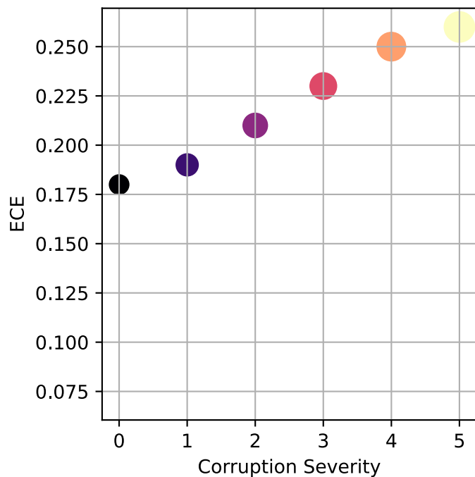
ResNet-18
