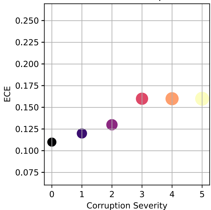
Manifold Mixup
