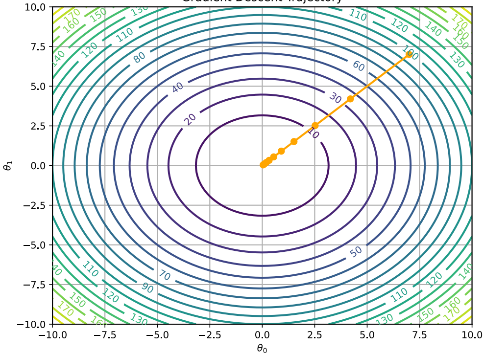
Gradient Descent Trajectory
