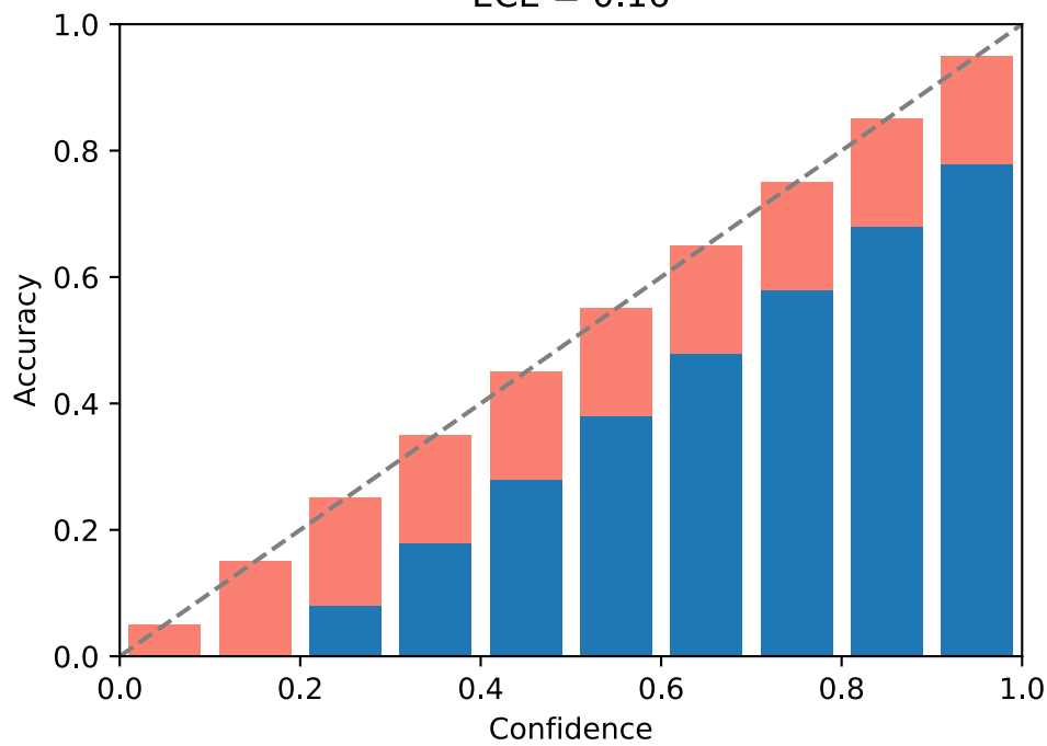
Manifold Mixup ECE = 0.16
