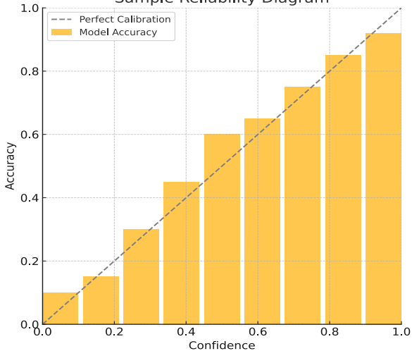
Sample Reliability Diagram
