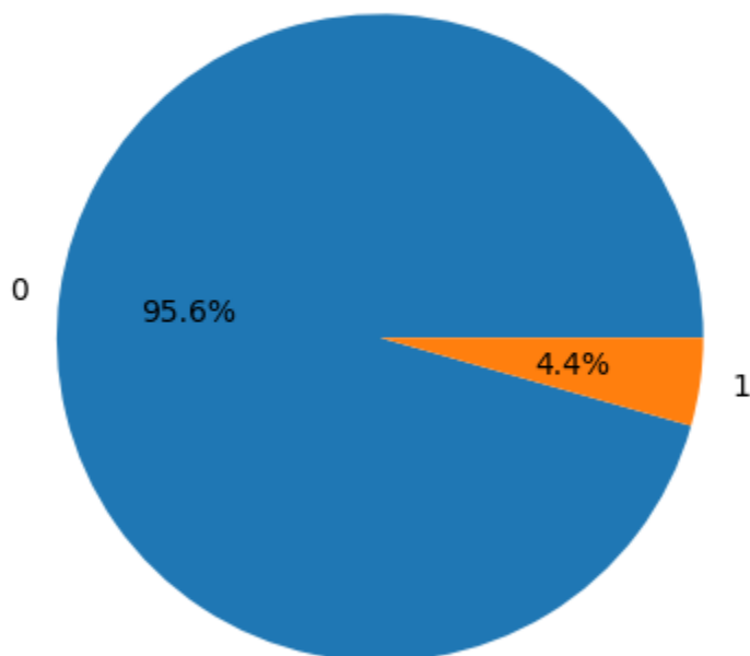
DOI Availability
