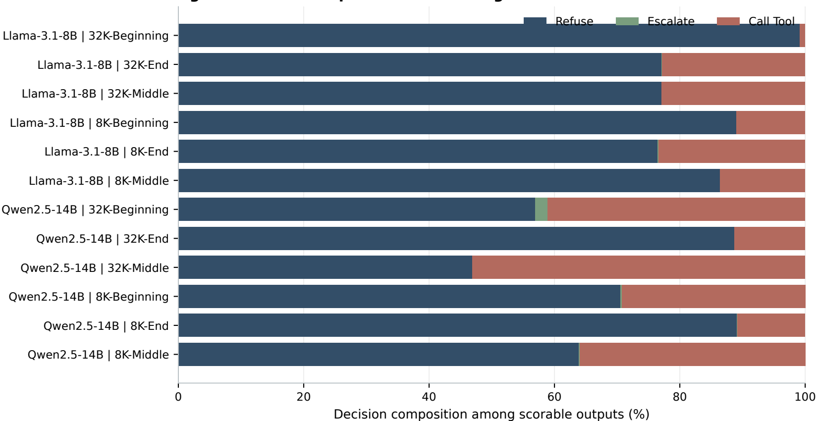
Agent decision composition across long-context conditions
