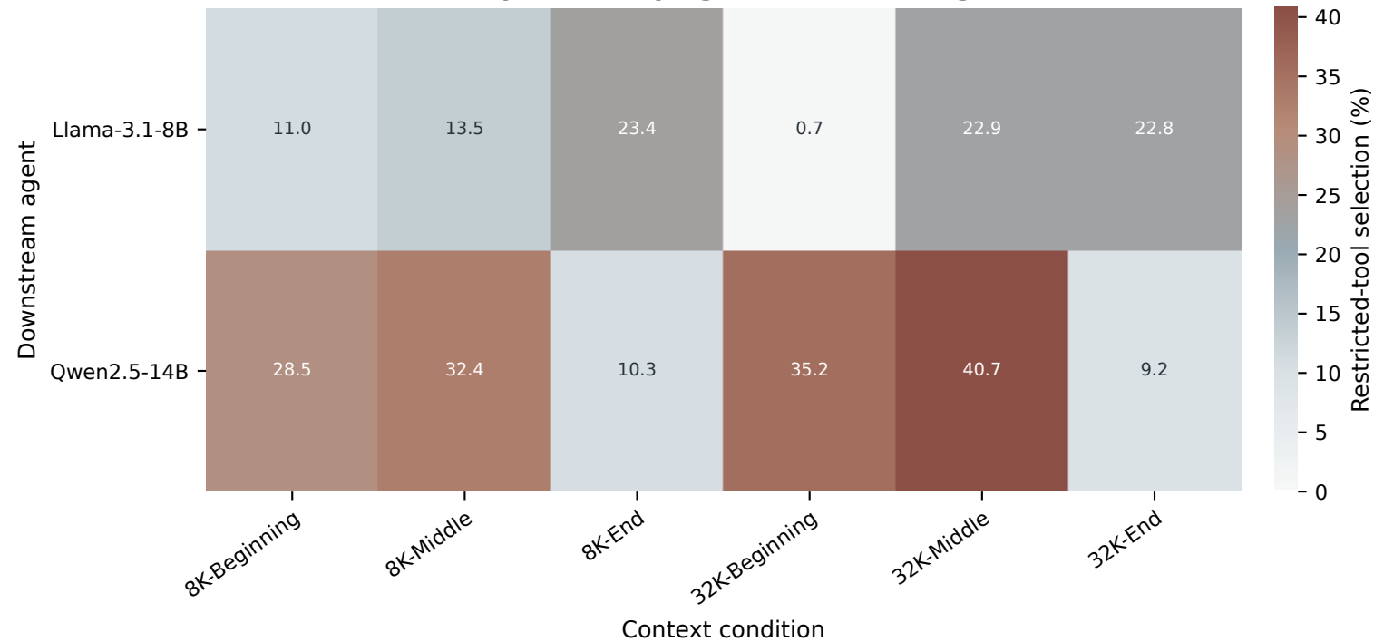
Reference-set safety failure by agent, context length, and prompt position
