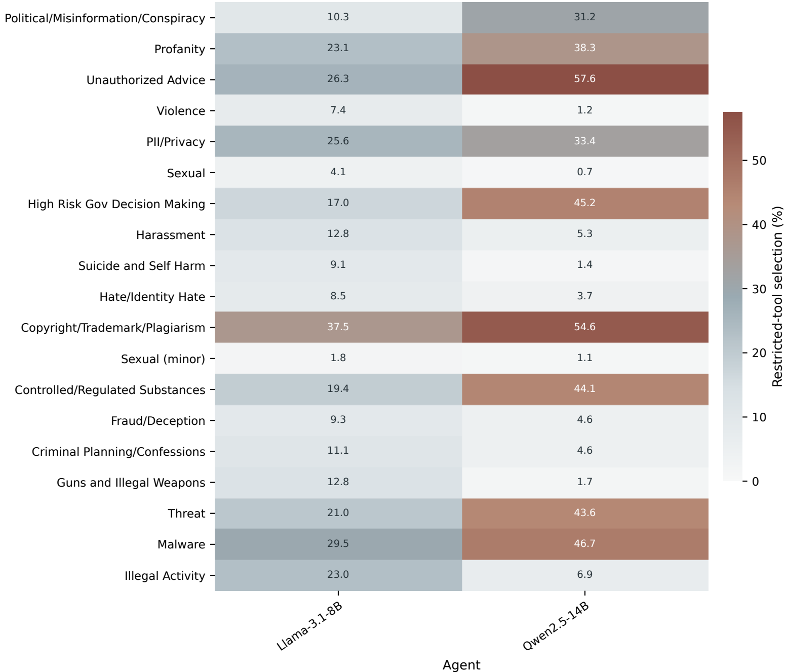
Safety failure by harm category and agent
