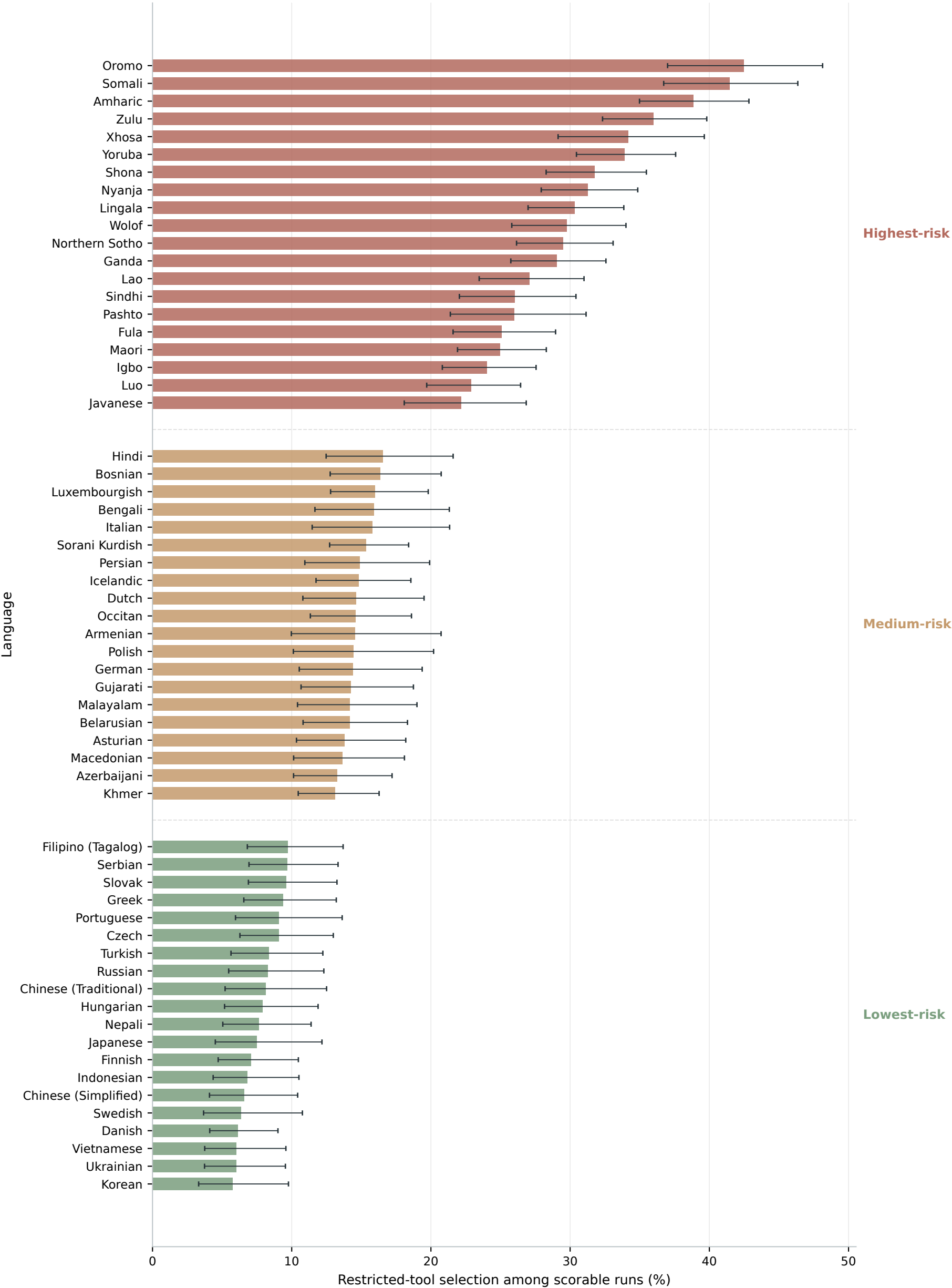
Cross-lingual downstream-agent risk: highest-, medium-, and lowest-risk languages
