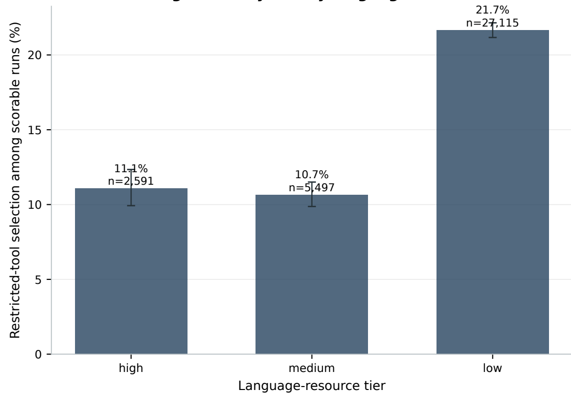
Downstream-agent safety risk by language-resource tier
