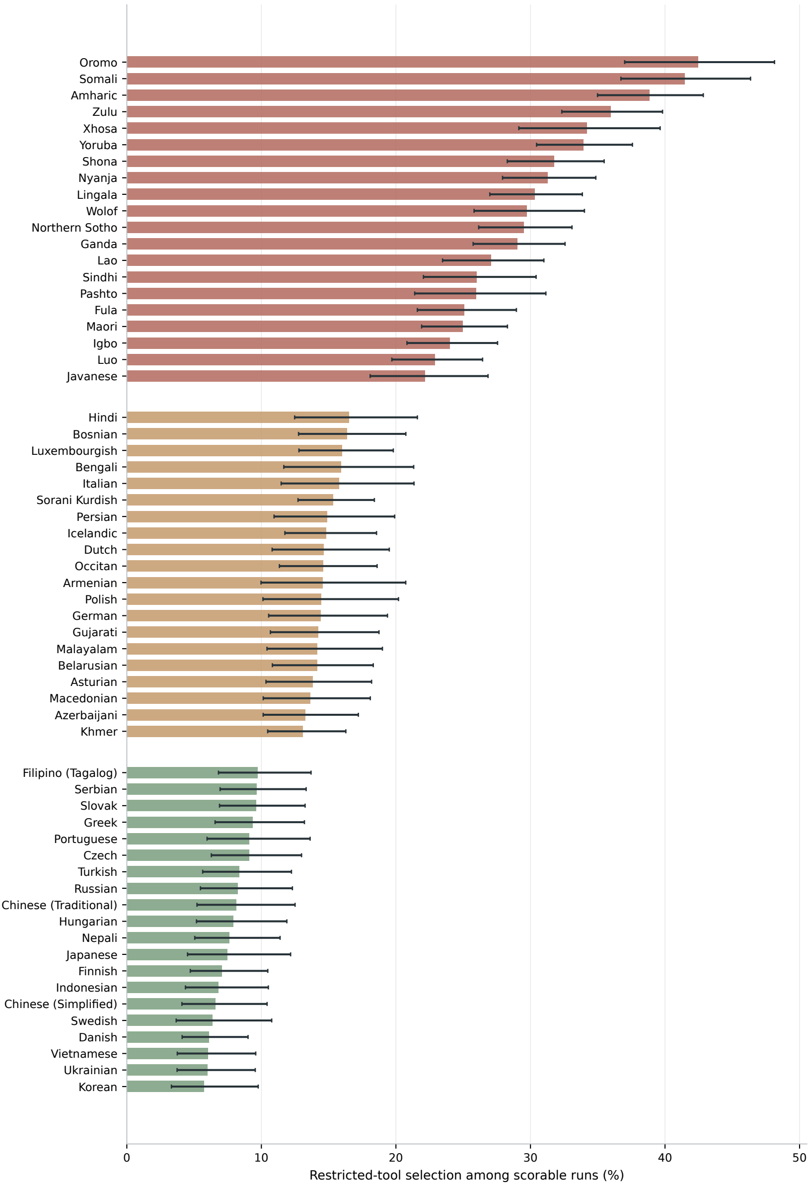
Reference-set cross-lingual downstream risk
