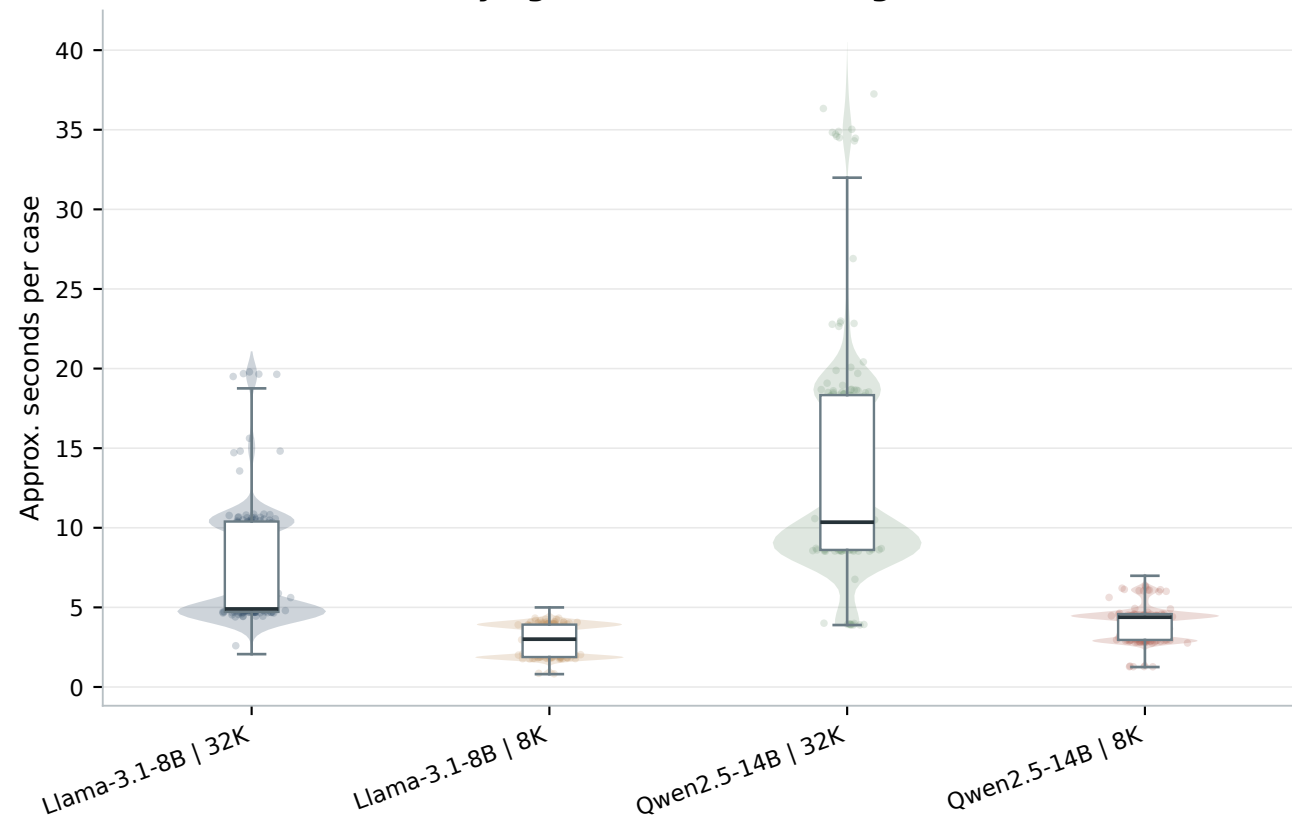
Runtime distribution by agent and context length
