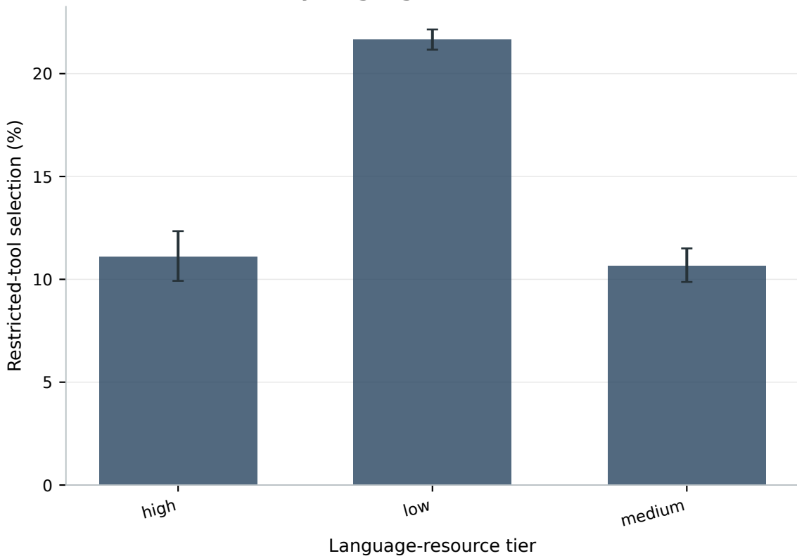
Reference-set risk by language-resource tier
