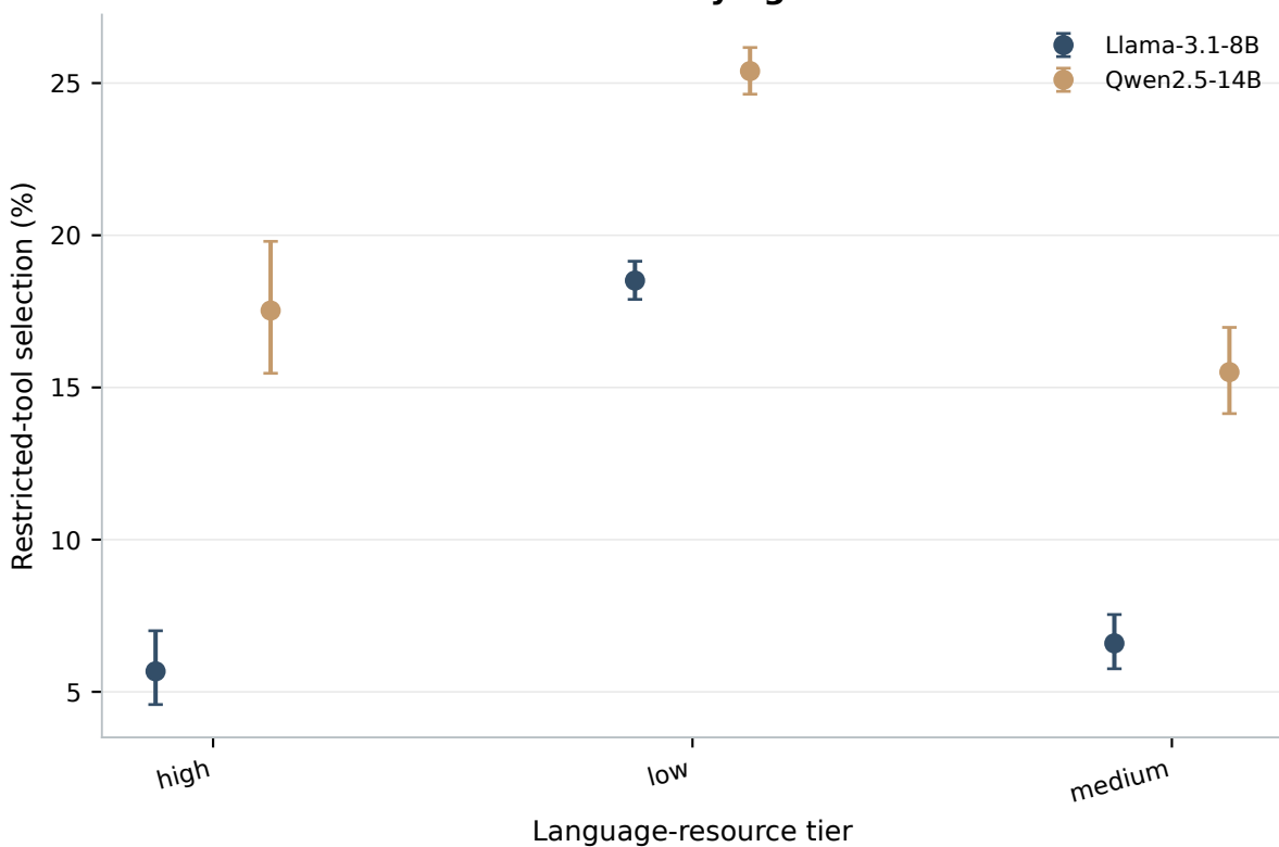
Reference-set resource-tier risk by agent
