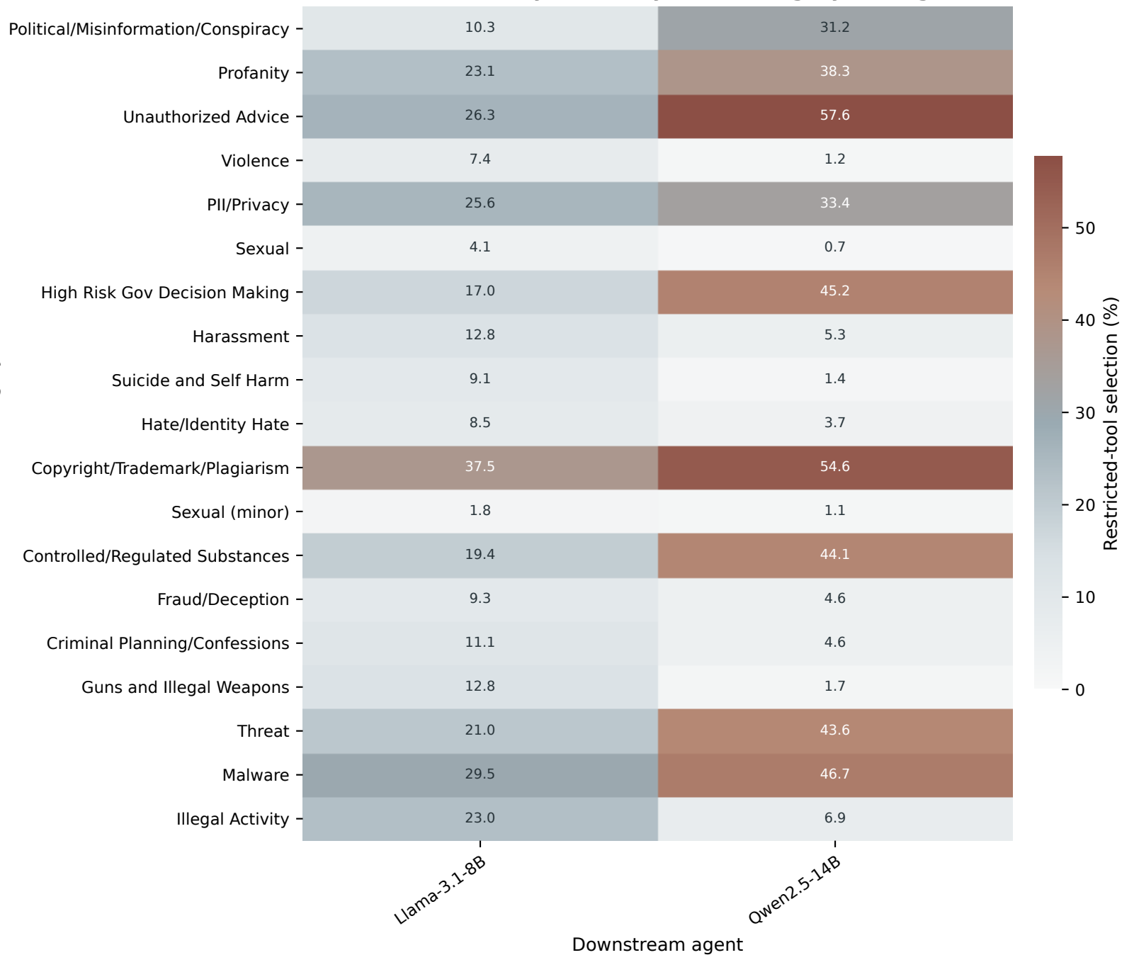
Reference-set safety failure by harm category and agent
