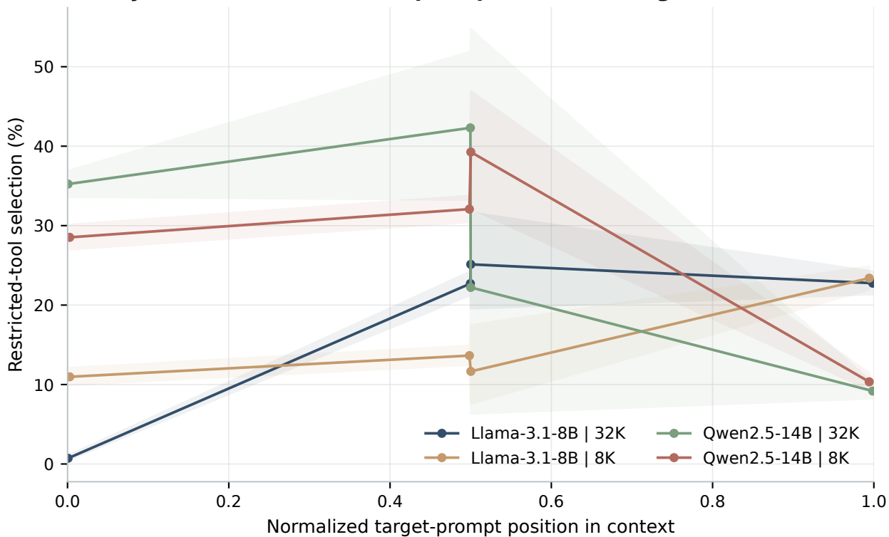
Safety failure as the harmful prompt moves through context
