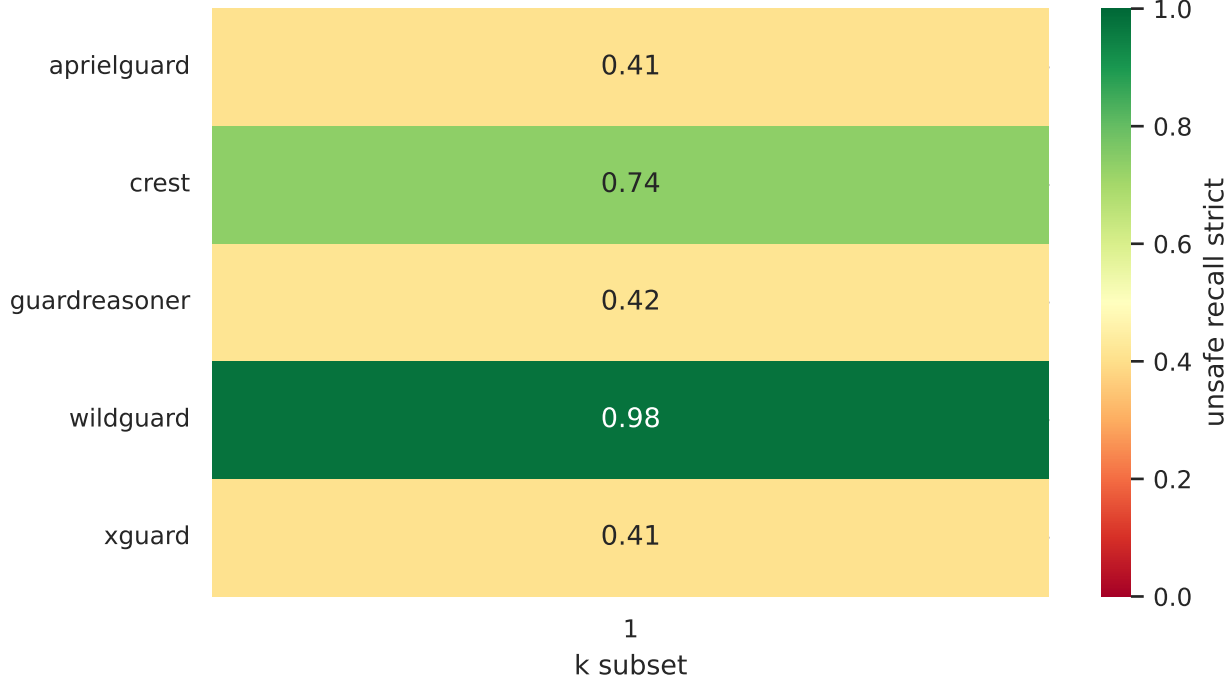
Strict unsafe recall across k
