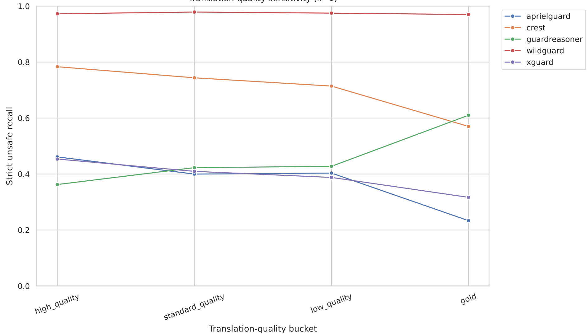
Translation-quality sensitivity (k=1)
