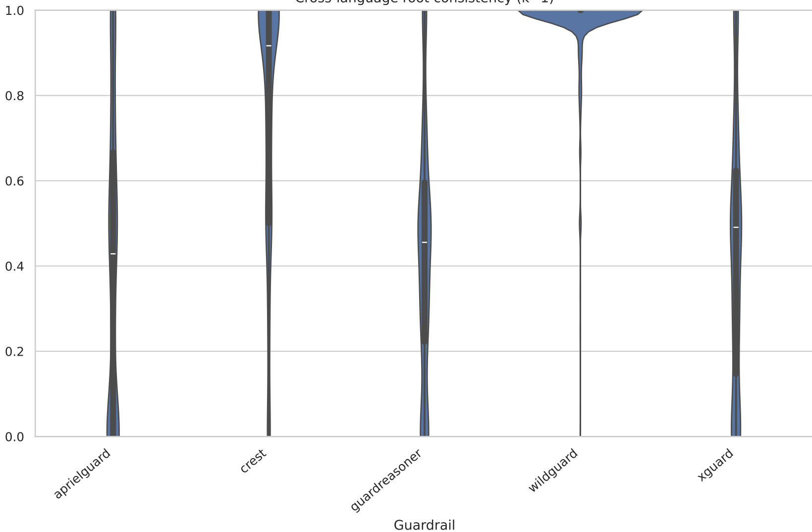
Cross-language root consistency (k=1)
