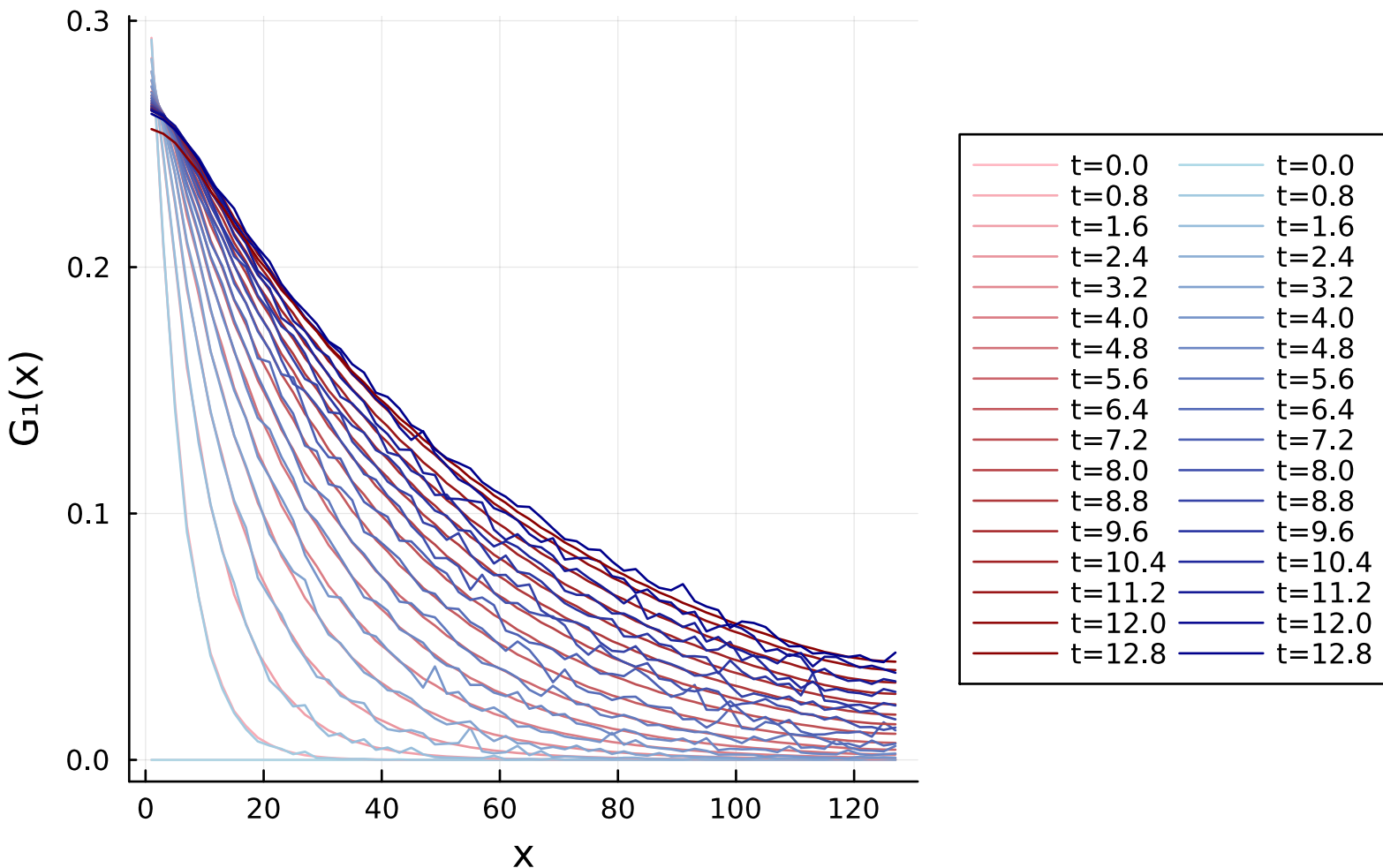
L=128 Renyi-1 TCI (red) vs. sampled (blue)
