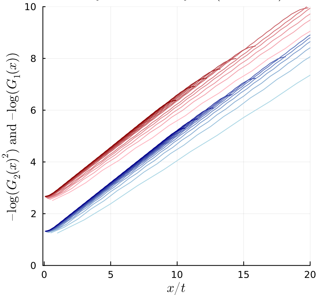
Renyi-1 vs. Renyi-2 ( L = 128 )
