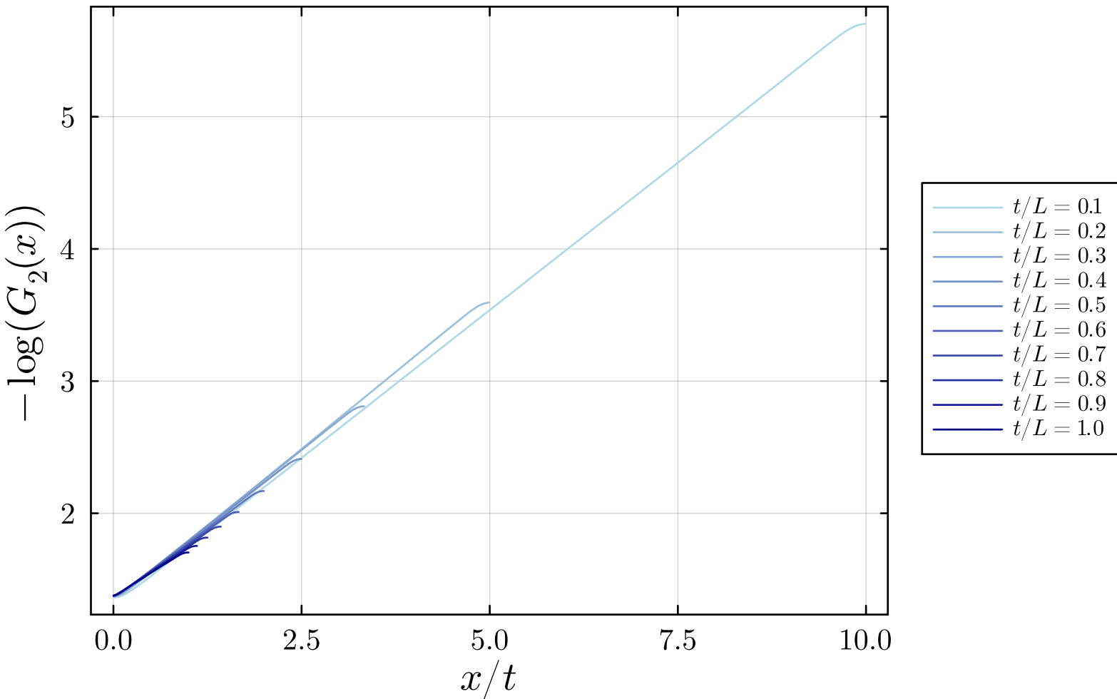
Renyi-2 correlations ( L = 1024 )
