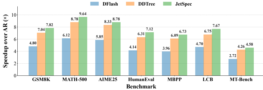
Figure 1: End-to-end decoding speedup over standard autoregressive decoding on H100 GPUs across math, coding, and chat benchmarks. DFlash denotes the original block-parallel drafting method, DDTree is tree-based variant of DFlash, and JetSpec denotes our method. Both employ a tree budget of 256 tokens using Algorithm 1.
