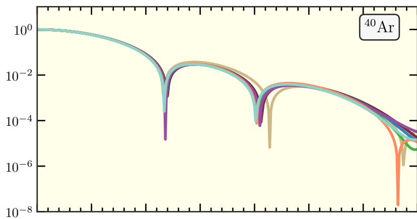
Charge Form Factor
