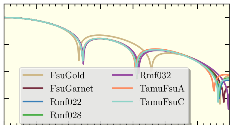
Weak Form Factor
