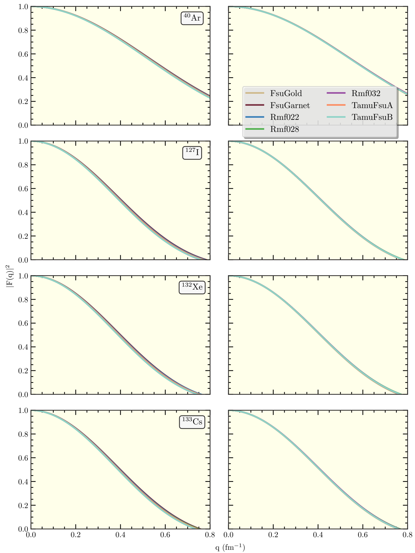
Charge Form Factor
