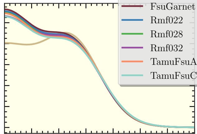
Neutron Density
