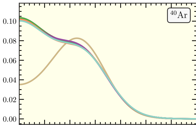
Proton Density
