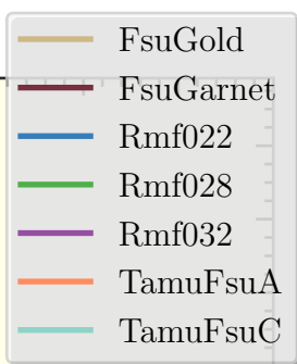
Neutron Density
