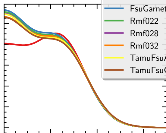
Neutron Density
