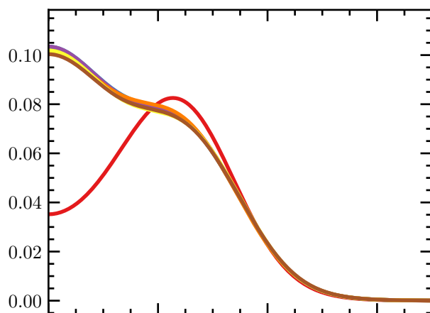
Proton Density
