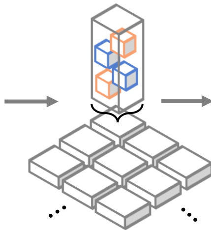
BEV Aggregation
