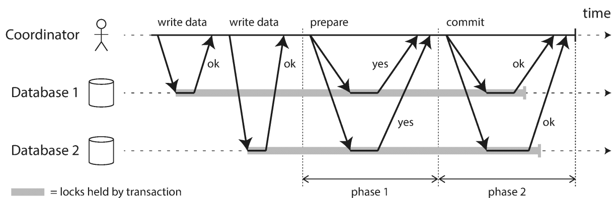
Figure 9-9. A successful execution of two-phase commit (2PC).
