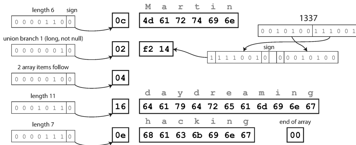
Figure 4-5. Example record encoded using Avro.
