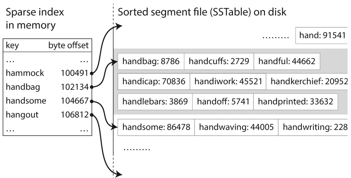
Figure 3-5. An SSTable with an in-memory index.
