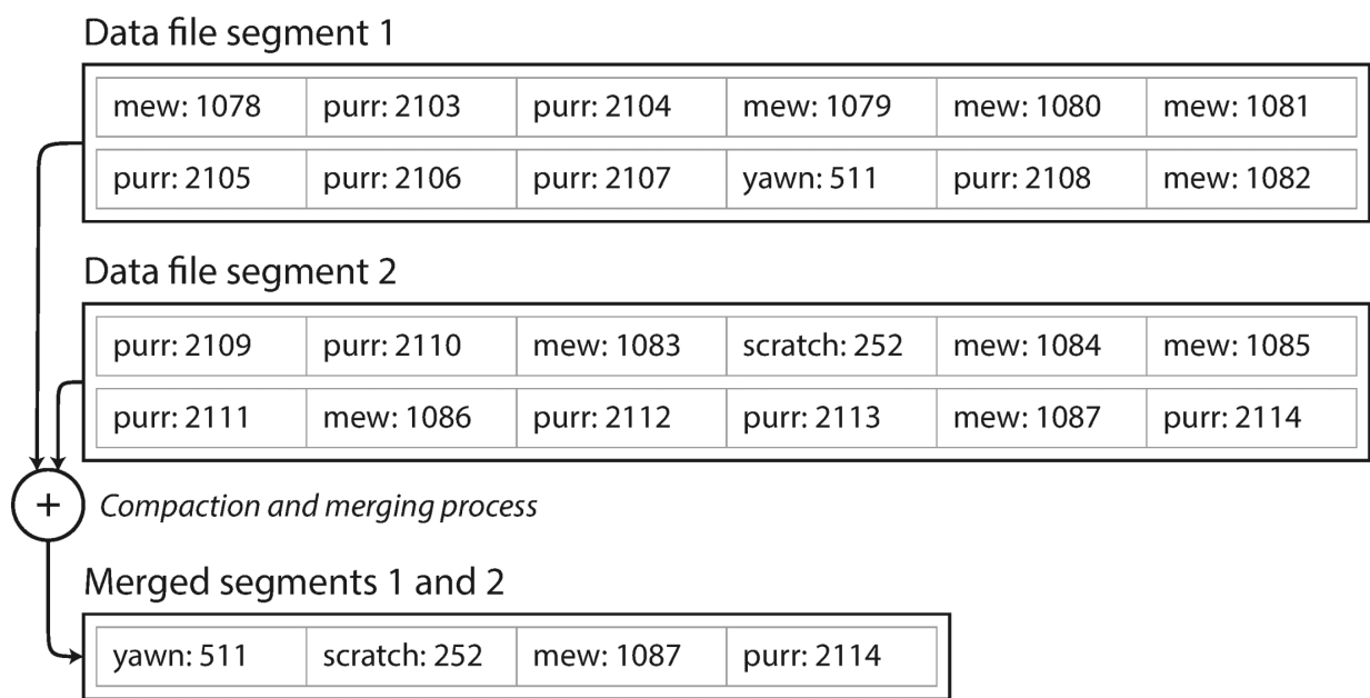
Figure 3-3. Performing compaction and segment merging simultaneously.
