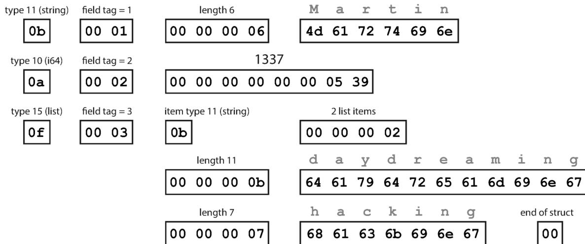
Figure 4-2. Example record encoded using Thrift's BinaryProtocol.
