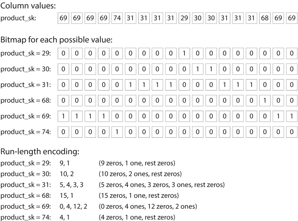
Figure 3-11. Compressed, bitmap-indexed storage of a single column.
