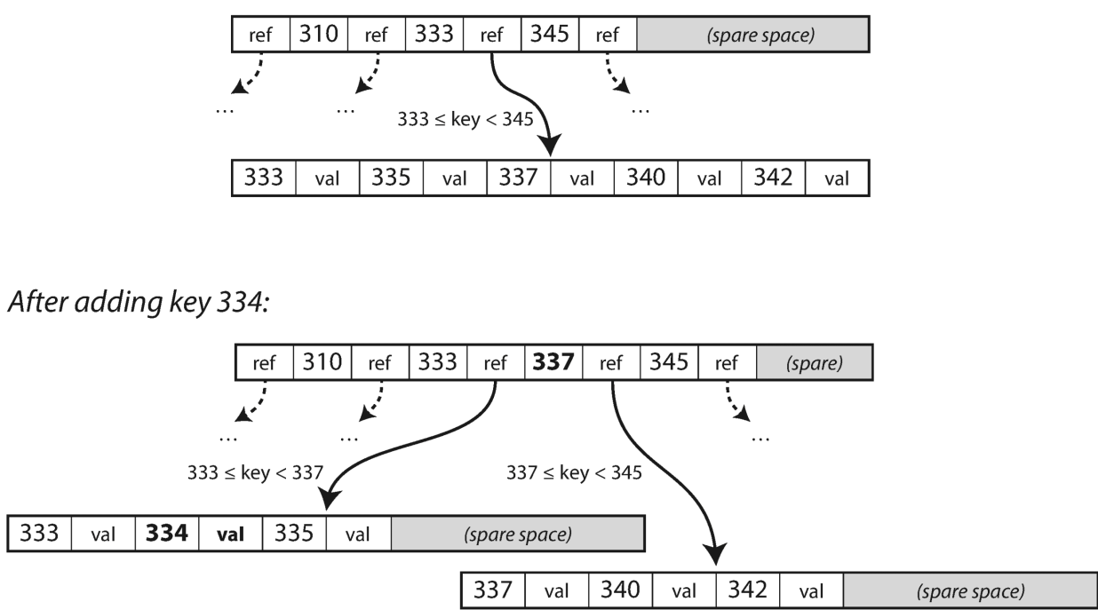
Figure 3-7. Growing a B-tree by splitting a page.
