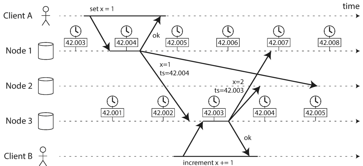
Figure 8-3. The write by client B is causally later than the write by client A, but B's write has an earlier timestamp.
