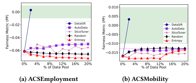
Figure 12: DATASIFT vs. baselines (Predictive Parity).
