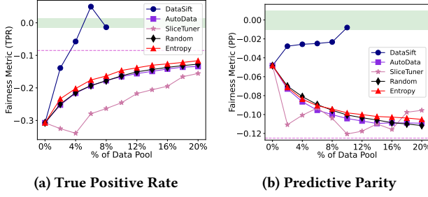
Figure 4: Evaluation of DATASIFT over different fairness metrics (ACSIIncome dataset, magenta dashed line: \mathcal{F}_{D_{train} \cup \mathcal{D}} ).
